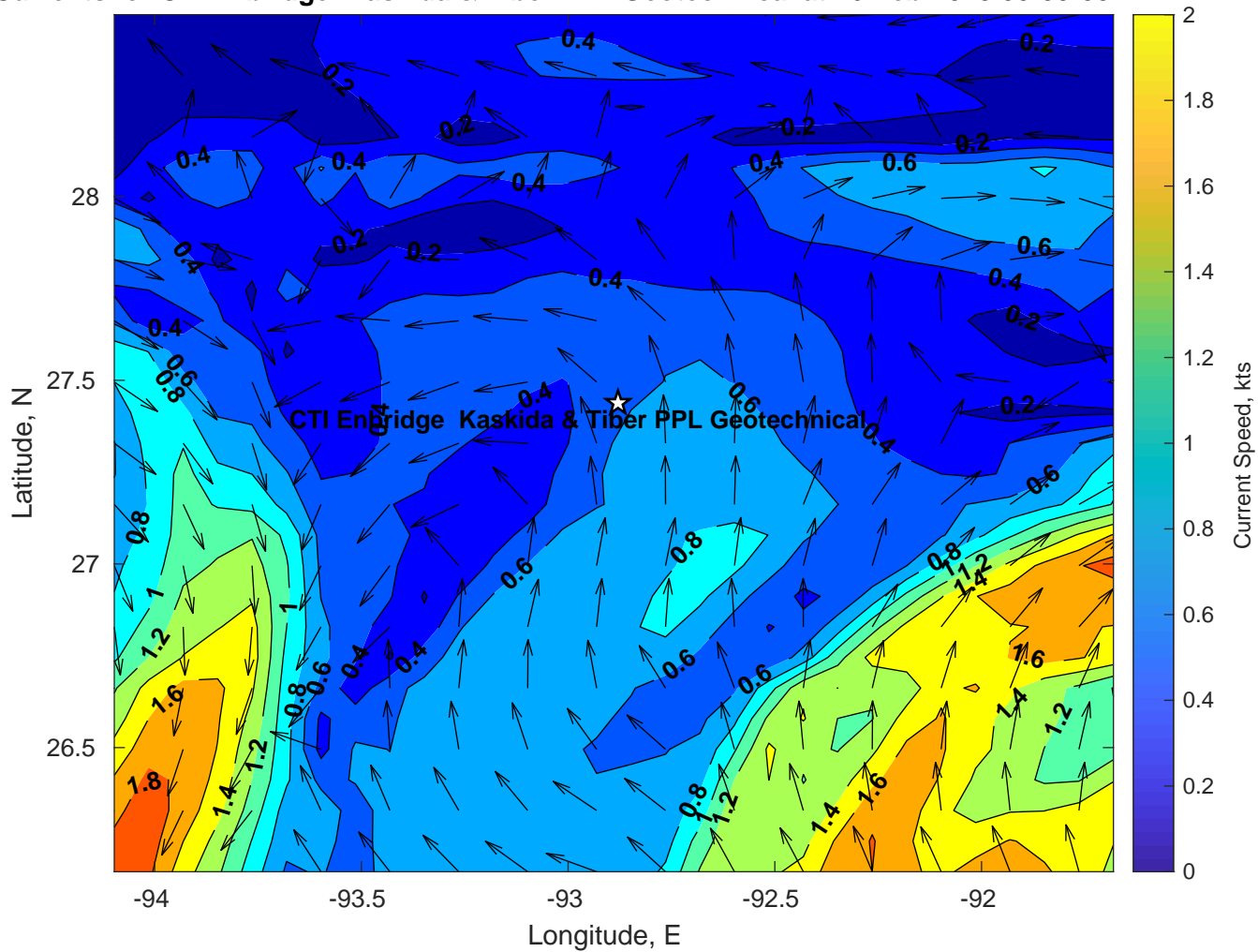
Surface Currents for CTI Enbridge Kaskida & Tiber PPL Geotechnical at 26-Feb-2025 00:00:00
