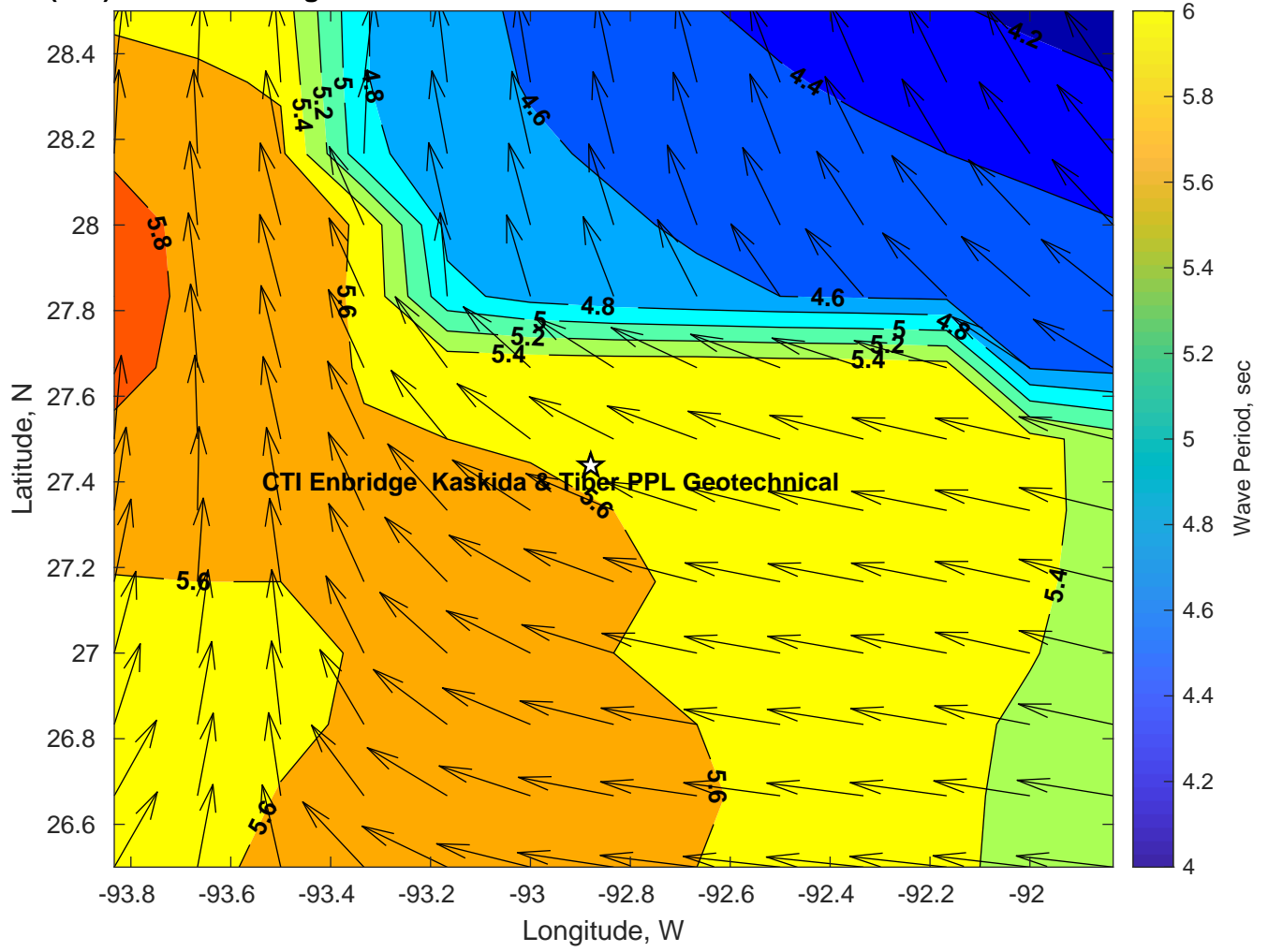
Wave Period (sec) for CTI Enbridge Kaskida & Tiber PPL Geotechnical at 27-Feb-2025 09:00:00
