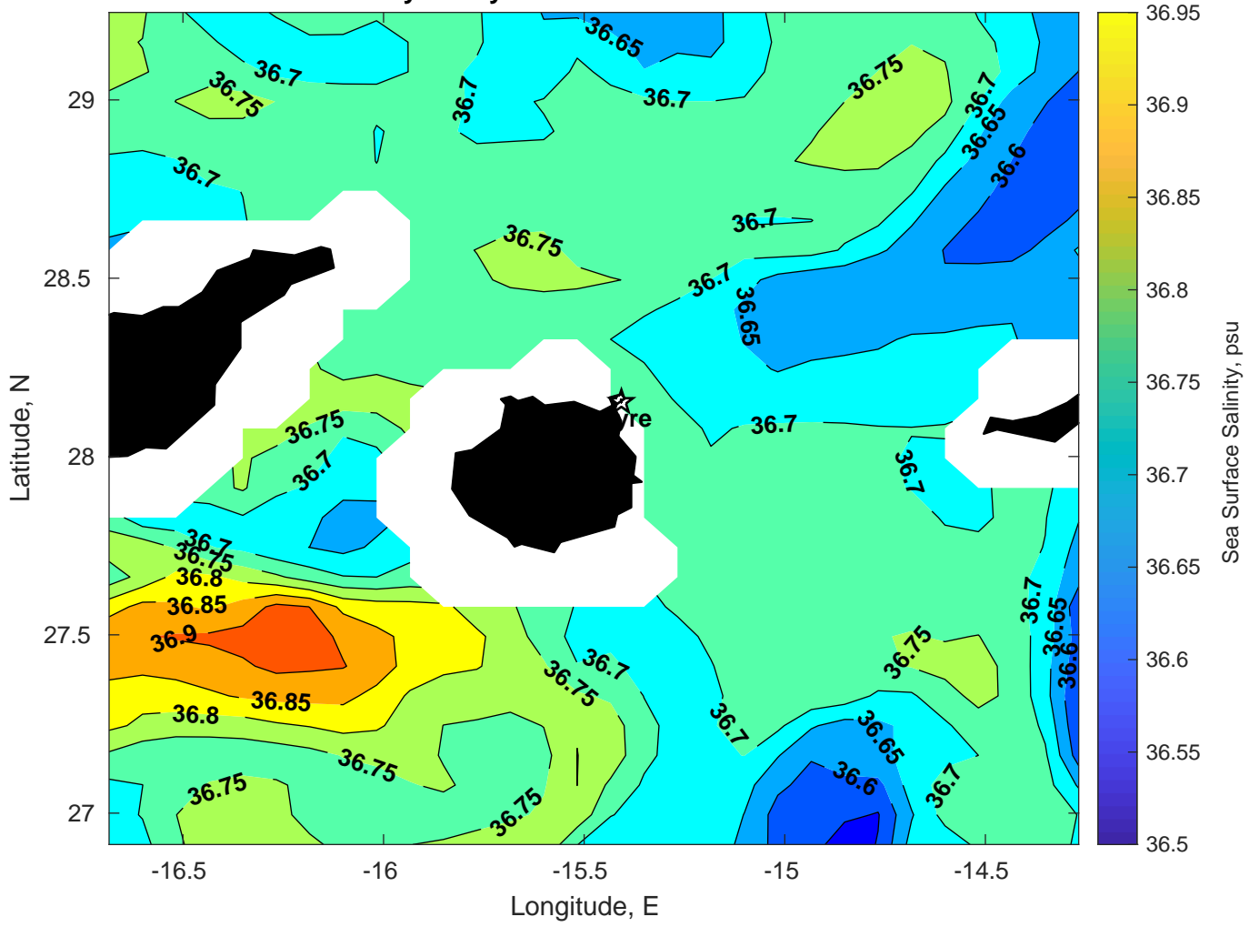
Surface Salinity for Gyre at 26-Feb-2025 00:00:00
