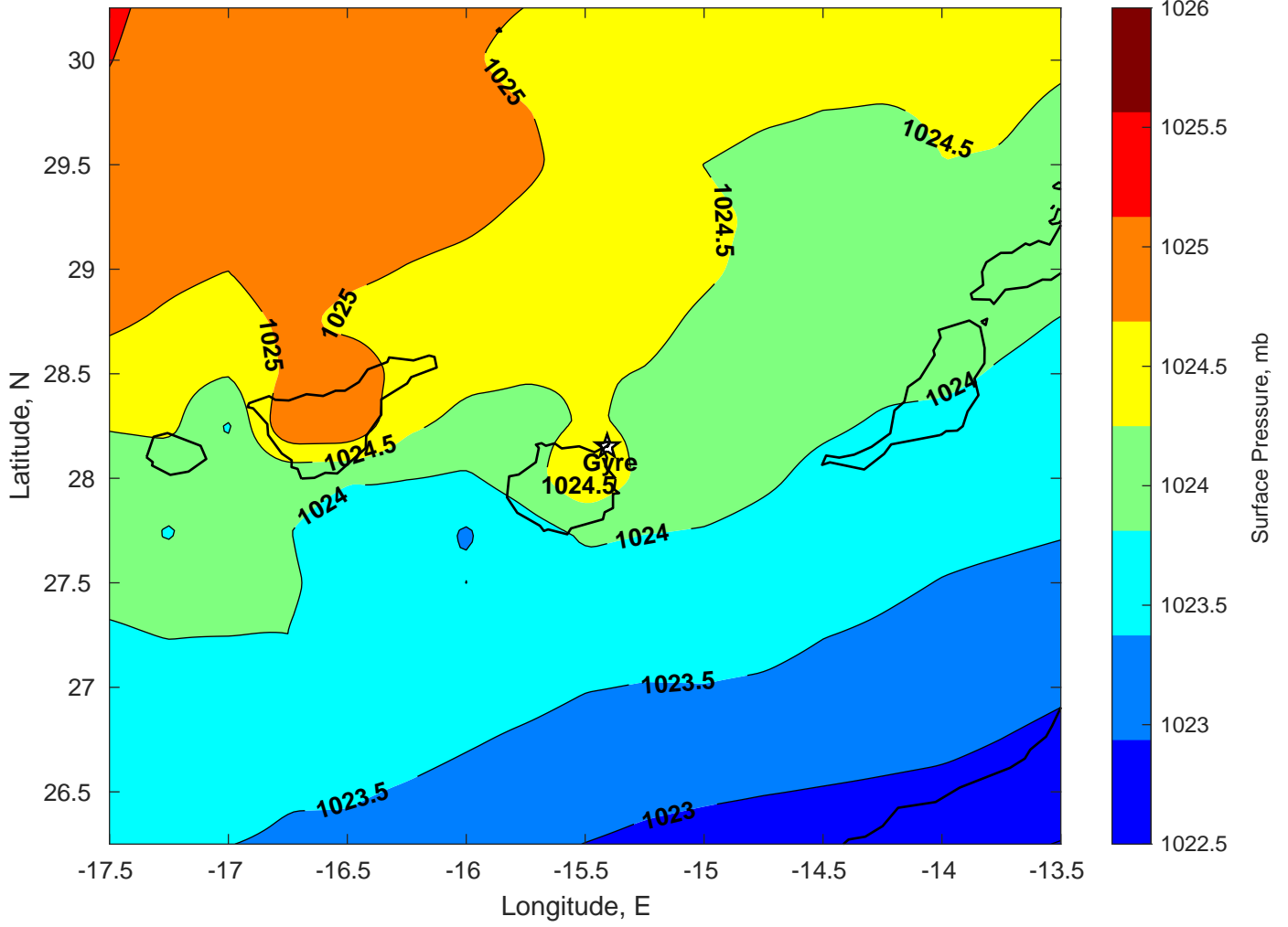
Surface Pressure (mb) for Gyre at 27-Feb-2025 00:00:00
