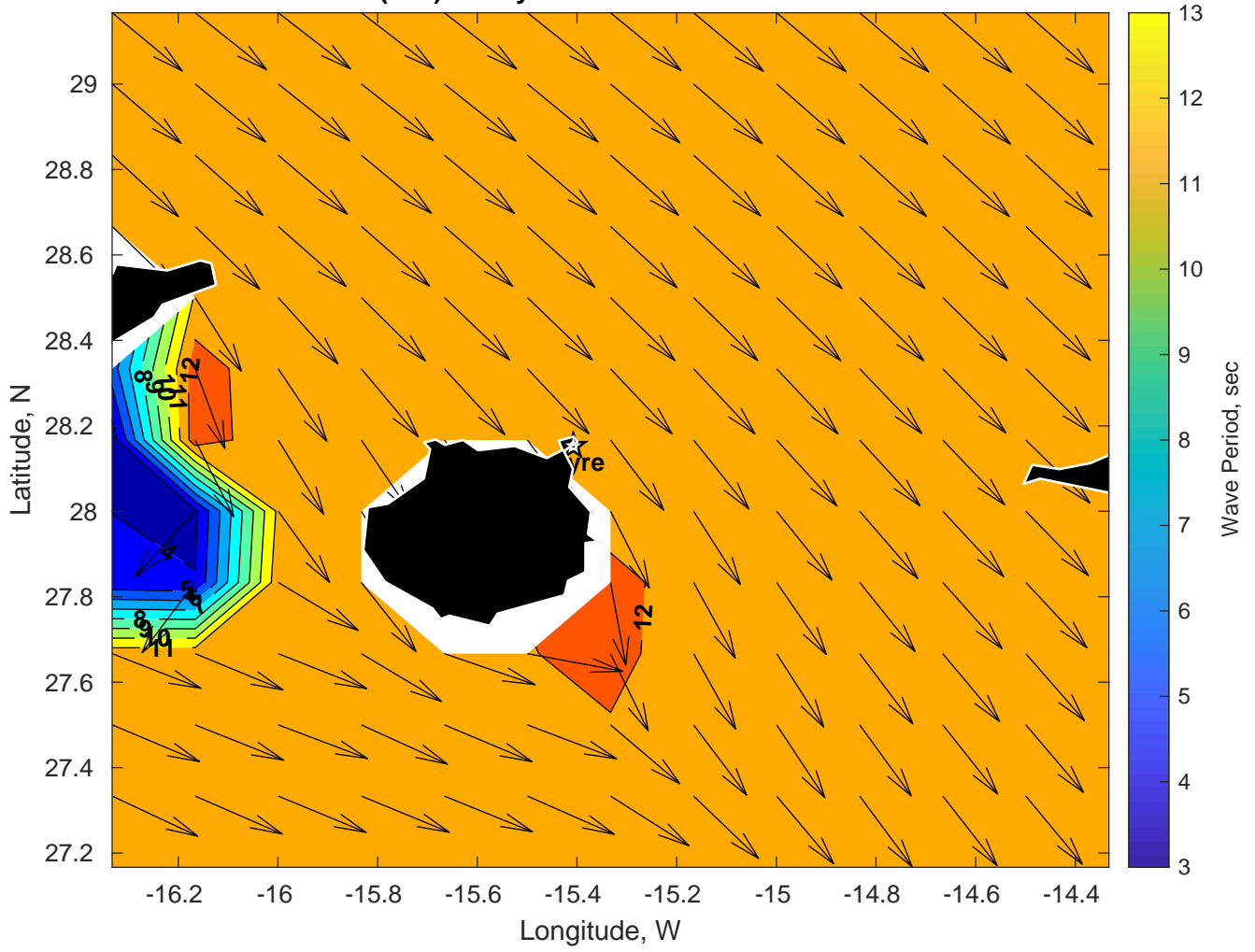
Wave Period (sec) for Gyre at 27-Feb-2025 09:00:00
