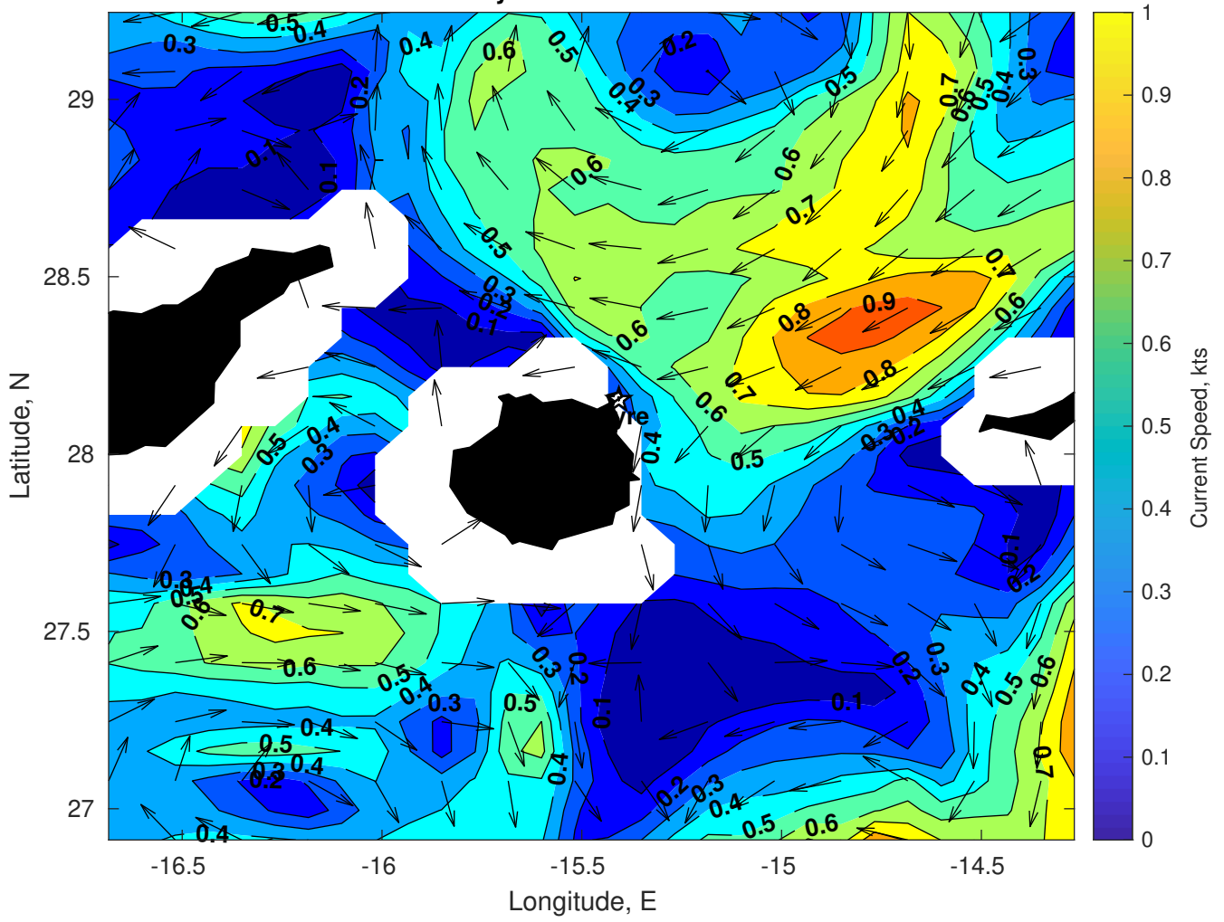
Surface Currents for Gyre at 26-Feb-2025 00:00:00
