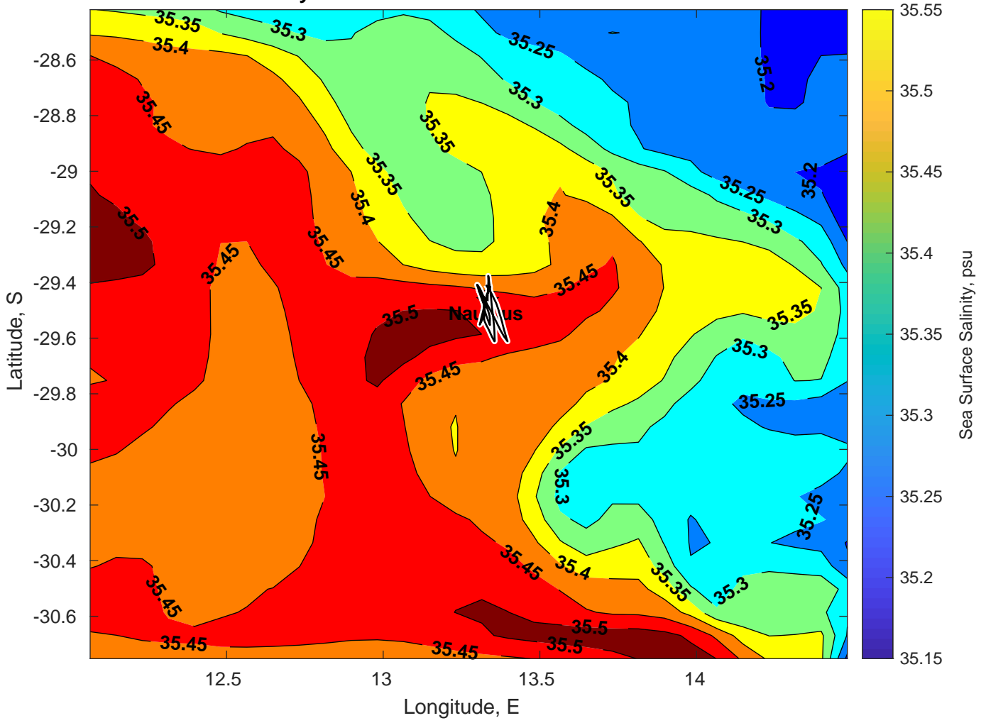
Surface Salinity for Nautilus at 26-Feb-2025 00:00:00
