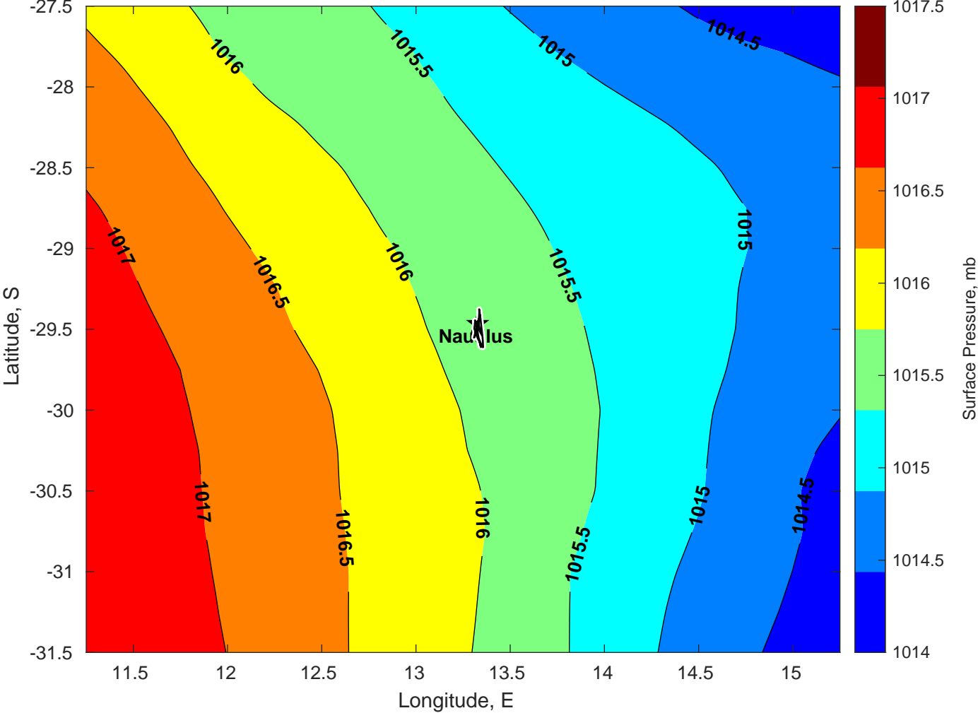
Surface Pressure (mb) for Nautilus at 01-Mar-2025 00:00:00
