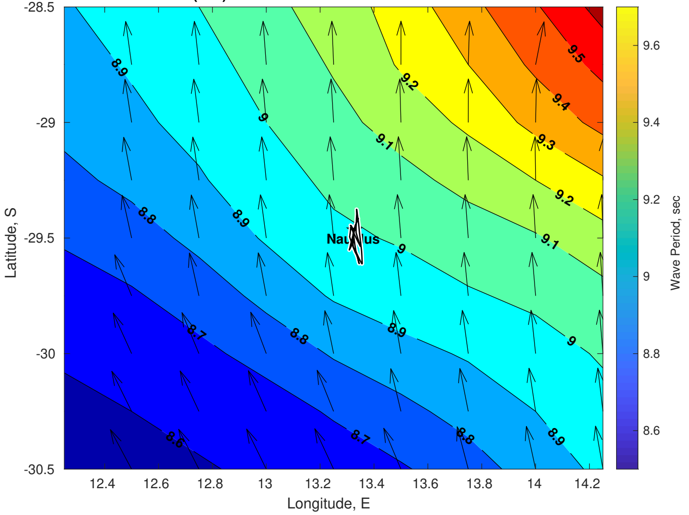
Wave Period (sec) for Nautilus at 27-Feb-2025 09:00:00
