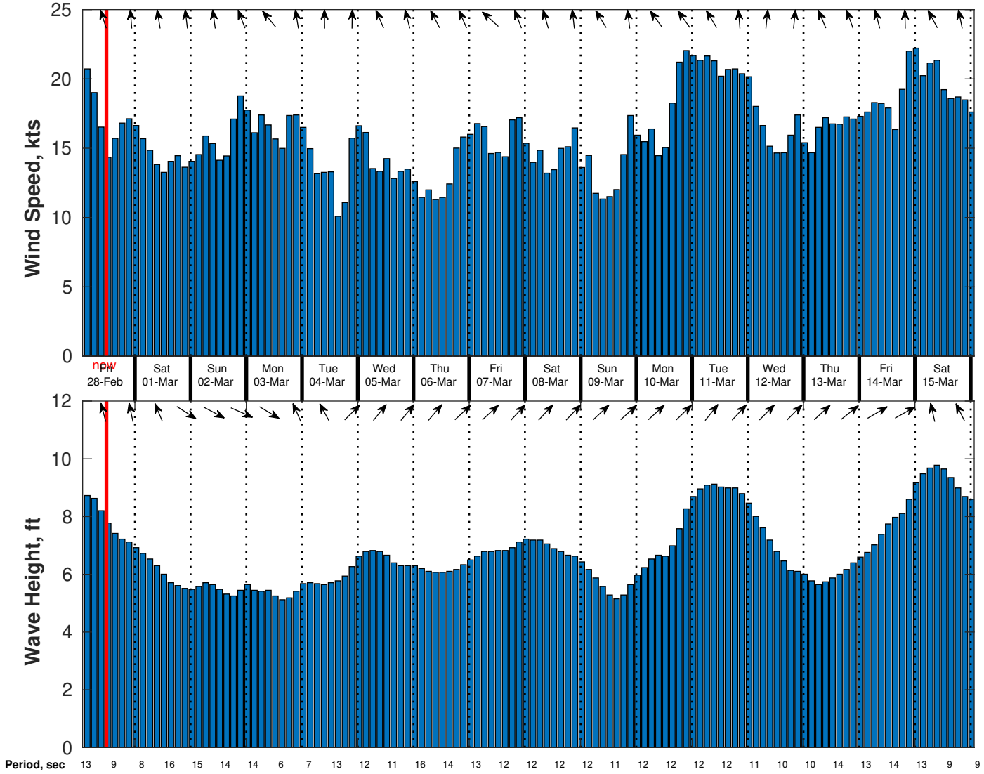
Wind & Wave Forecast for Nautilus from 27-Feb-2025 02:00:00 to 15-Mar-2025 02:00:00
