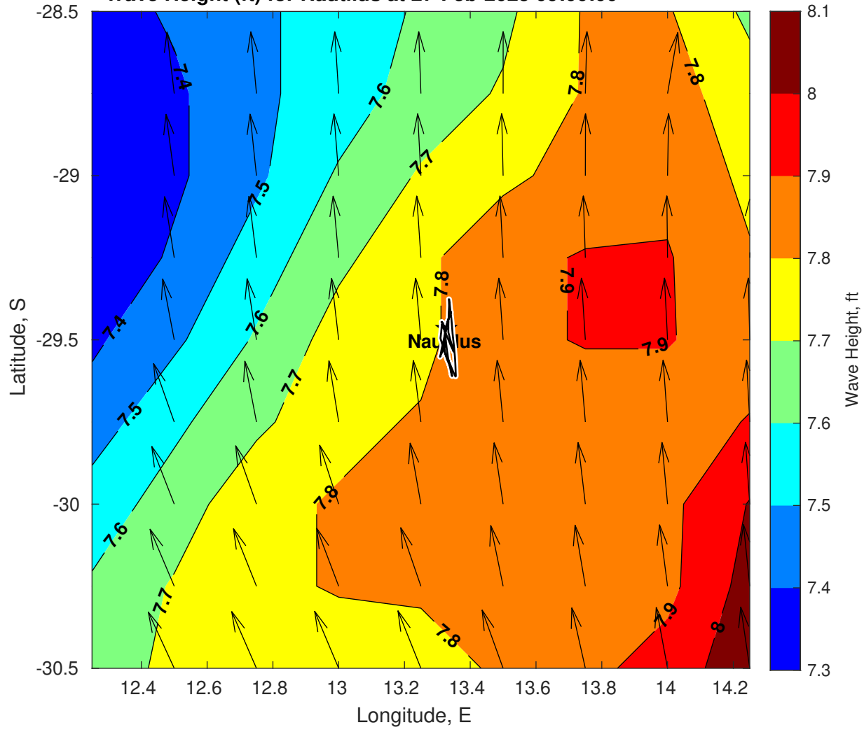
Wave Height (ft) for Nautilus at 27-Feb-2025 09:00:00
