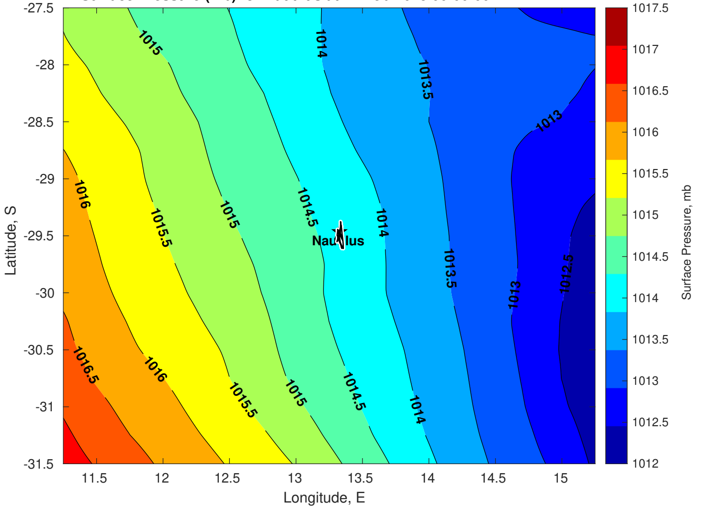
Surface Pressure (mb) for Nautilus at 27-Feb-2025 00:00:00
