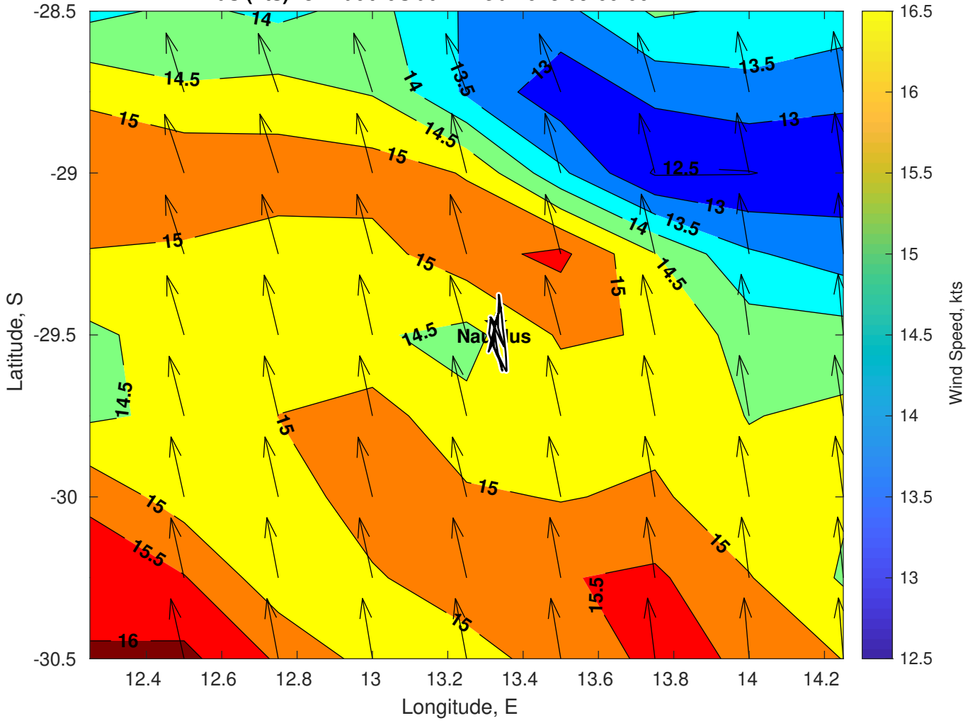
Winds (kts) for Nautilus at 27-Feb-2025 09:00:00
