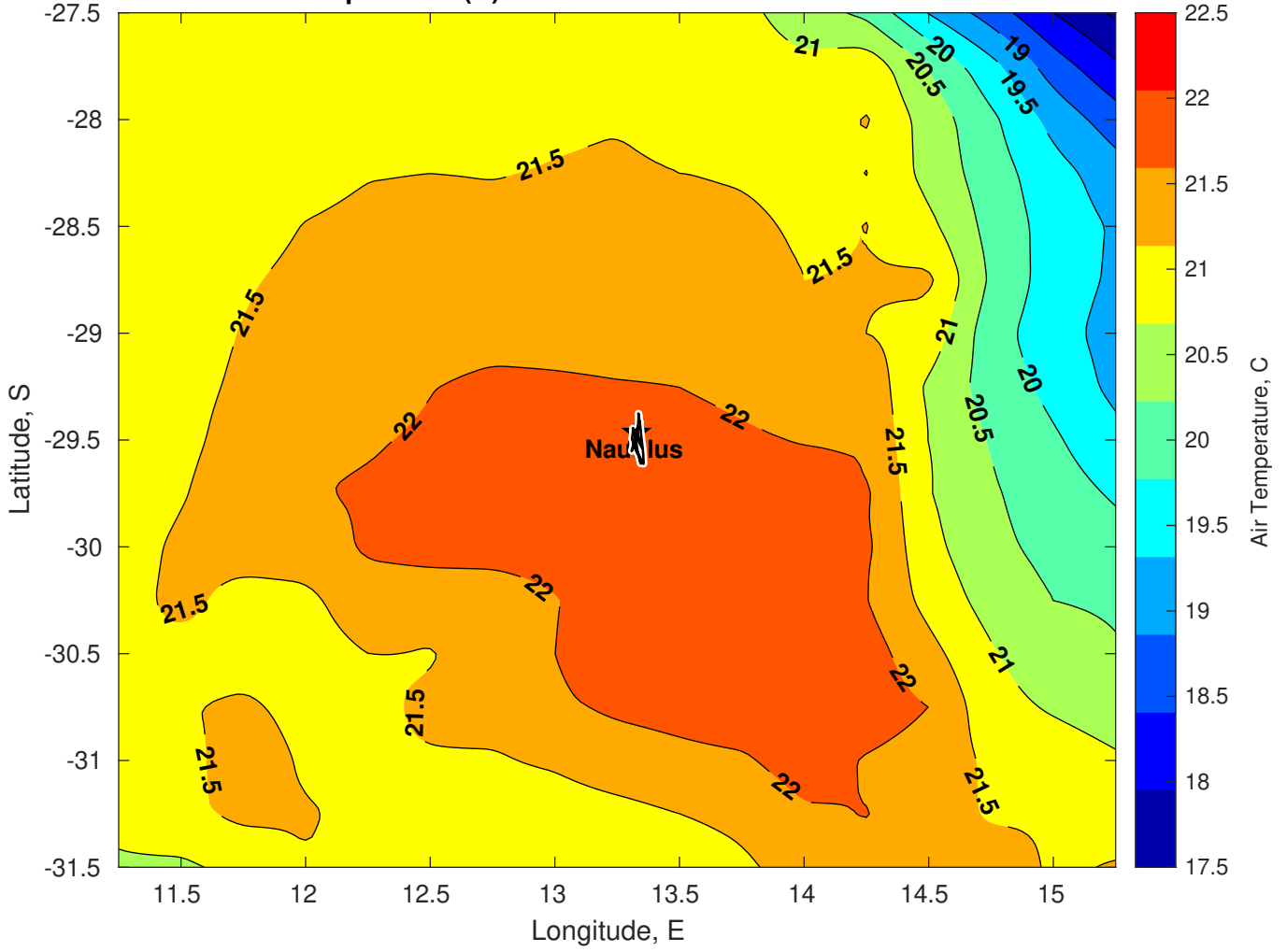
Air Temperature (C) for Nautilus at 27-Feb-2025
