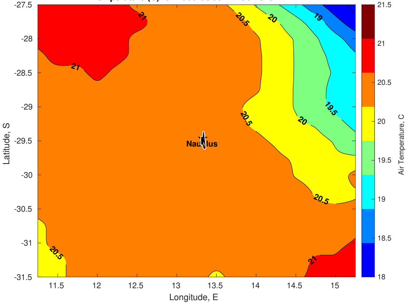
Air Temperature (C) for Nautilus at 27-Feb-2025
