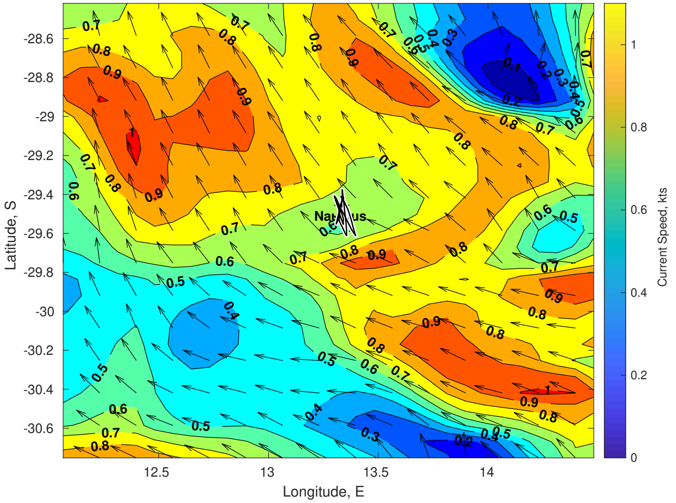
Surface Currents for Nautilus at 26-Feb-2025 00:00:00
