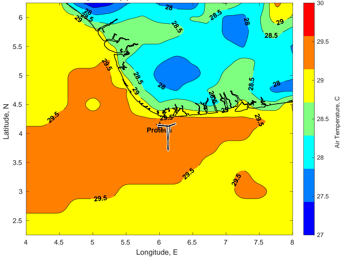
Air Temperature (C) for Proteus at 27-Feb-2025
