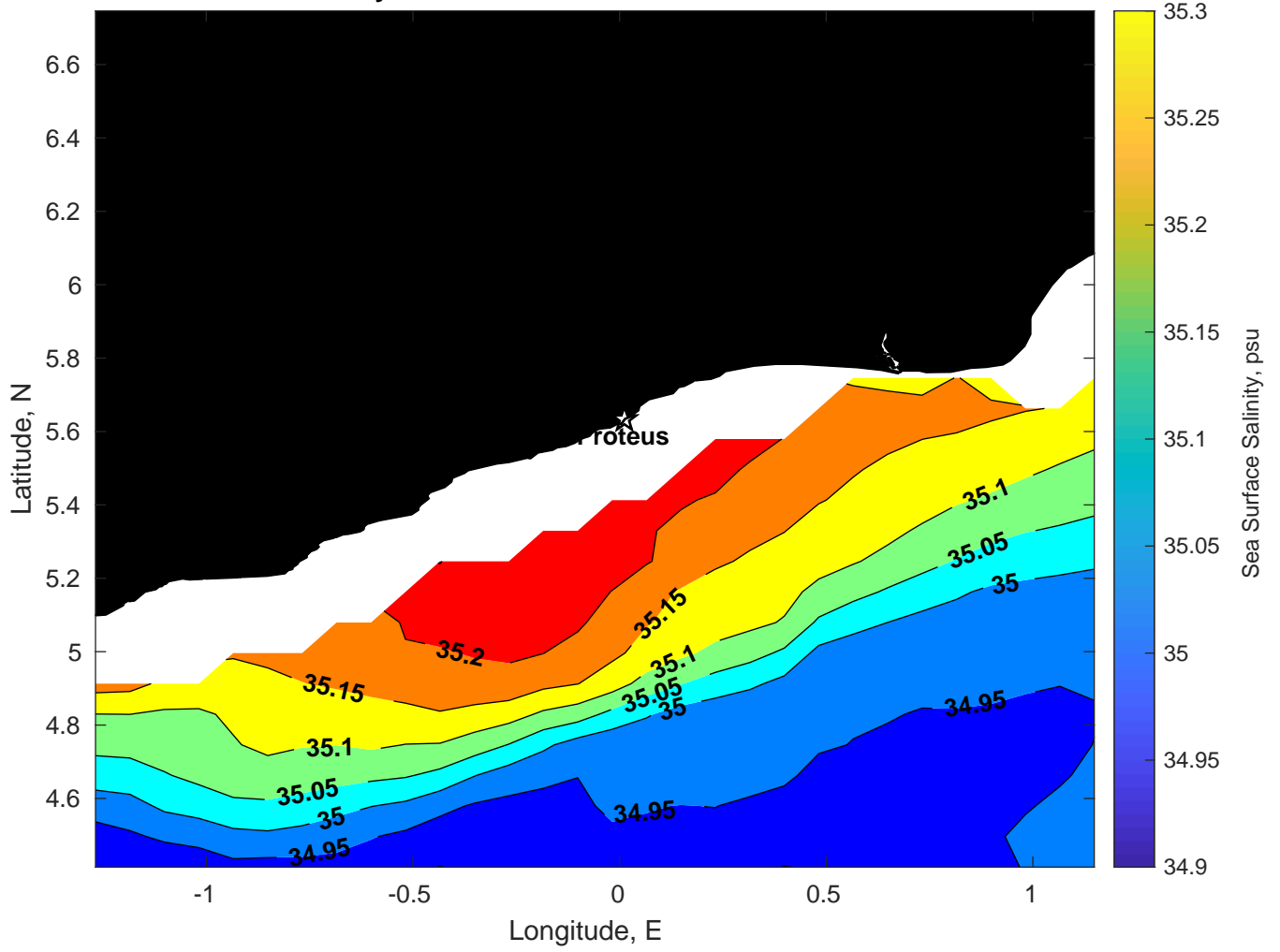
Surface Salinity for Proteus at 26-Feb-2025 00:00:00
