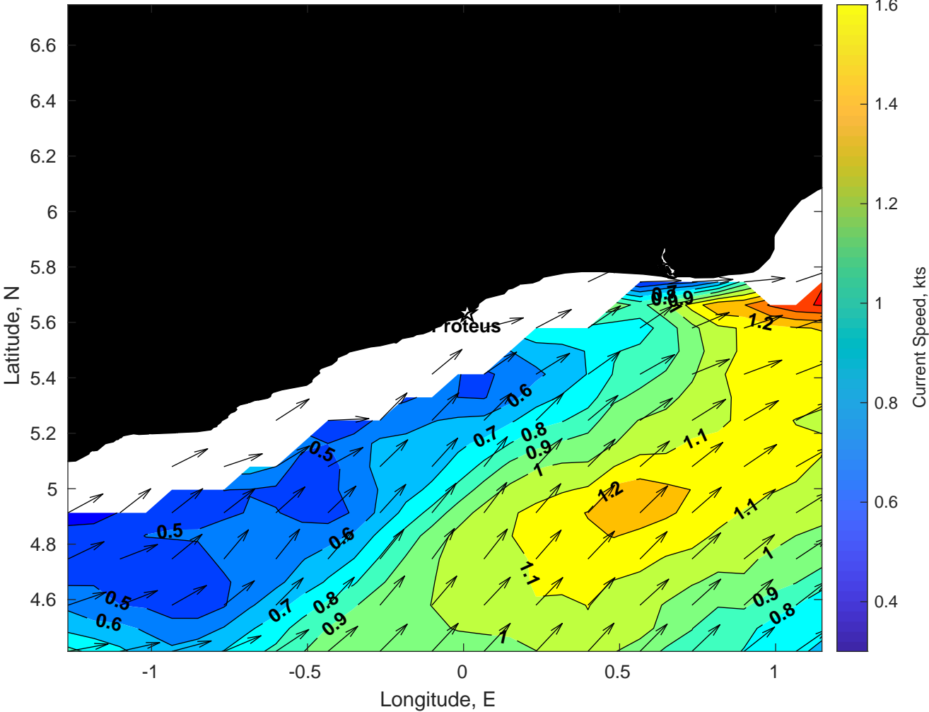
Surface Currents for Proteus at 26-Feb-2025 00:00:00
