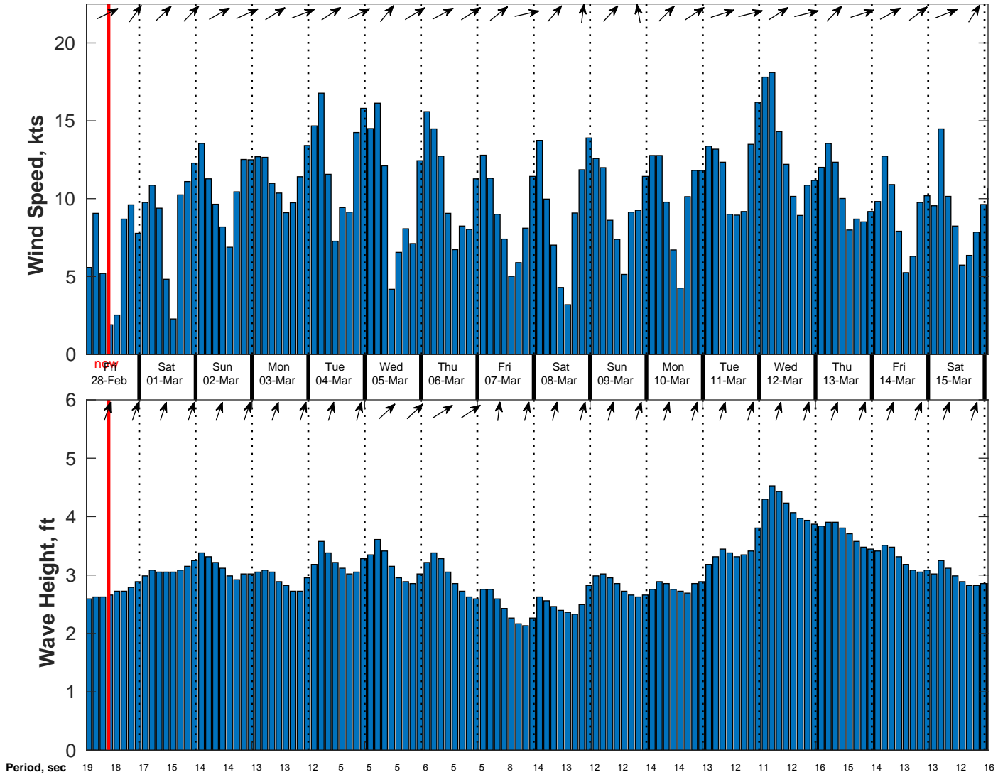
Wind & Wave Forecast for Proteus from 27-Feb-2025 01:00:00 to 15-Mar-2025 01:00:00
