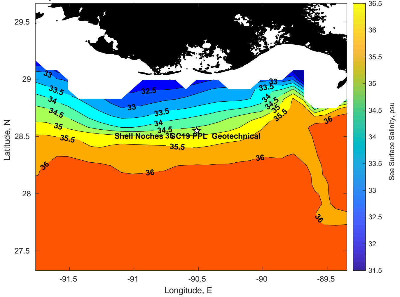
Surface Salinity for Shell Noches GC19 PPL Geotechnical at 26-Feb-2025 00:00:00
