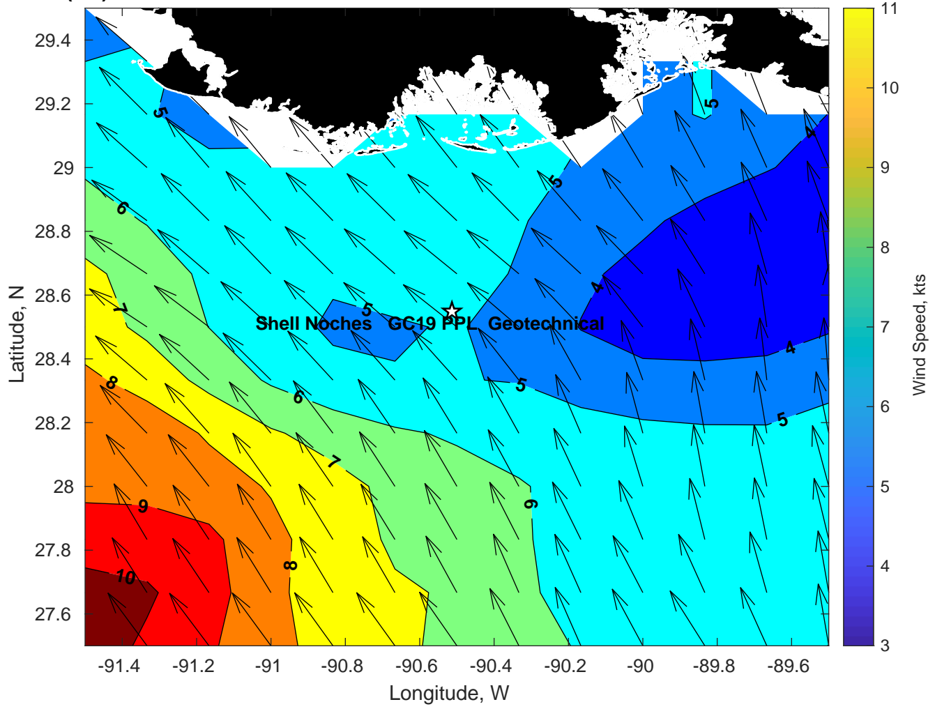
Winds (kts) for Shell Noches GC19 PPL Geotechnical at 27-Feb-2025 09:00:00
