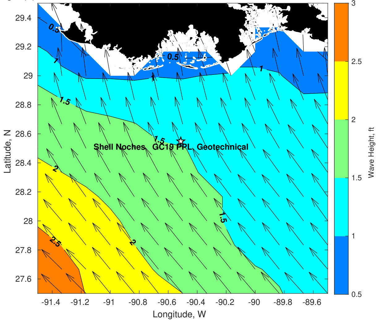
Wave Height (ft) for Shell Noches GC19 PPL Geotechnical at 27-Feb-2025 09:00:00
