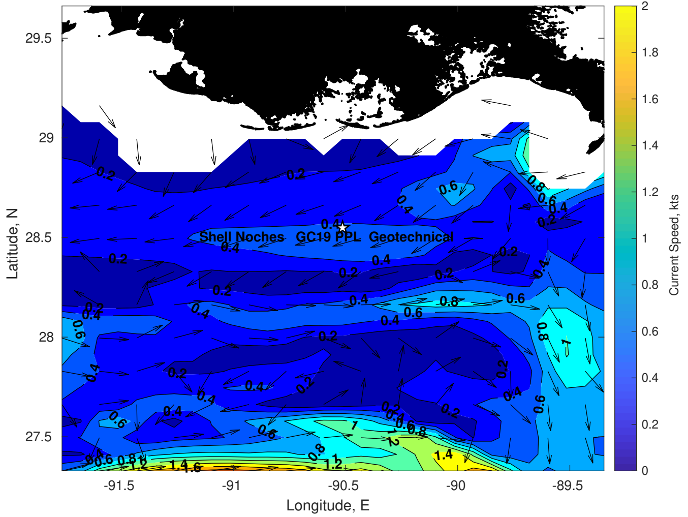
Surface Currents for Shell Noches GC19 PPL Geotechnical at 26-Feb-2025 00:00:00
