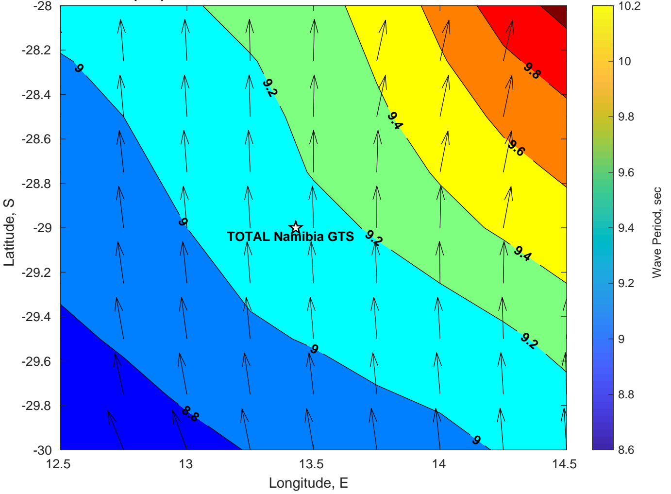
Wave Period (sec) for TOTAL Namibia GTS at 27-Feb-2025 09:00:00
