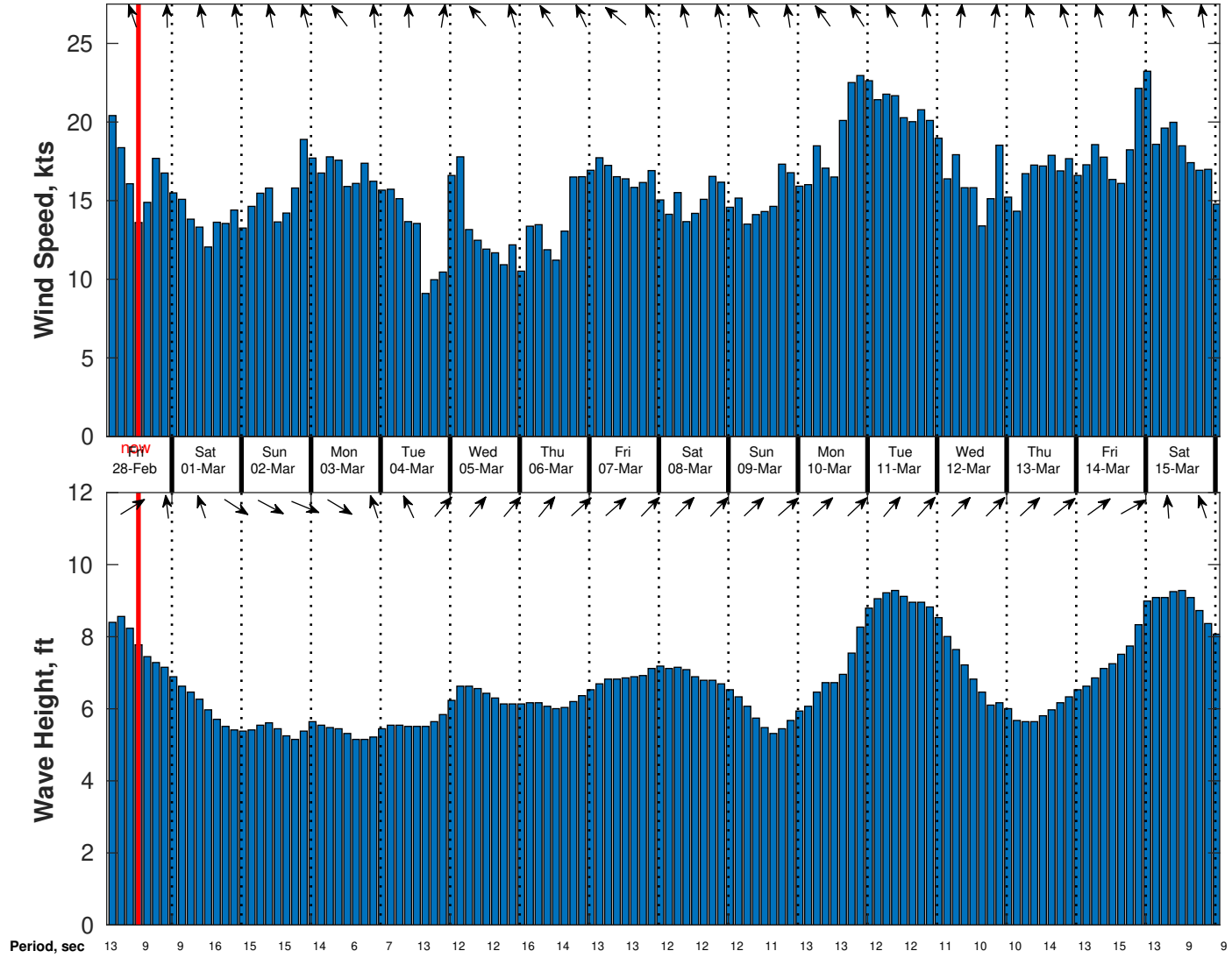
Wind & Wave Forecast for TOTAL Namibia GTS from 27-Feb-2025 02:00:00 to 15-Mar-2025 02:00:00
