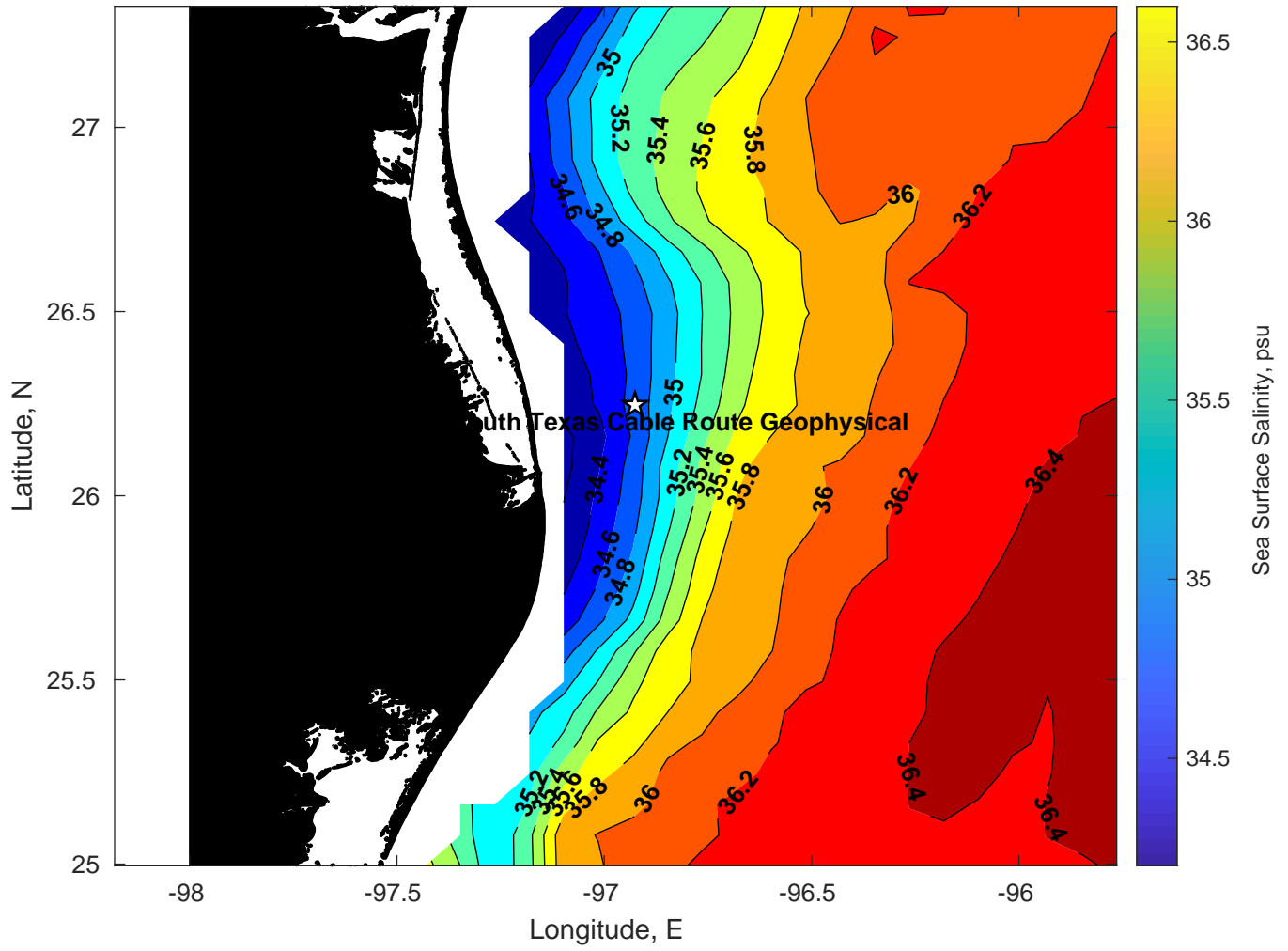
Surface Salinity for Tampnet P2378 South Texas Cable Route Geophysical at 26-Feb-2025 00:00:00
