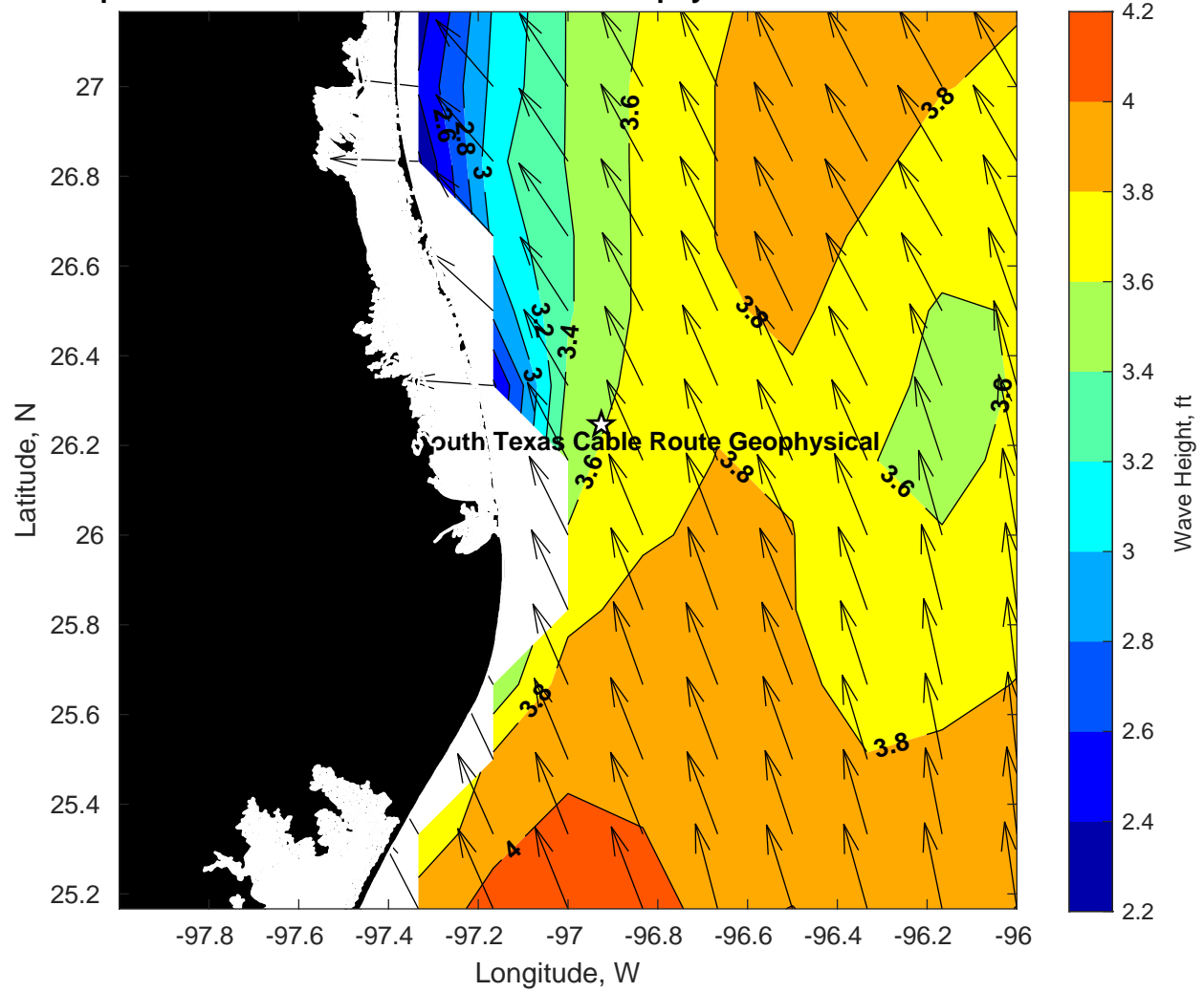
Wave Height (ft) for Tampnet P2378 South Texas Cable Route Geophysical at 27-Feb-2025 09:00:00
