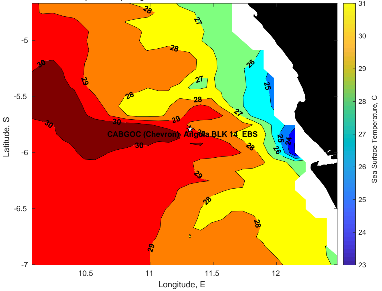
SST for CABGOC (Chevron) Angola BLK 14 EBS at 27-Feb-2025 00:00:00
