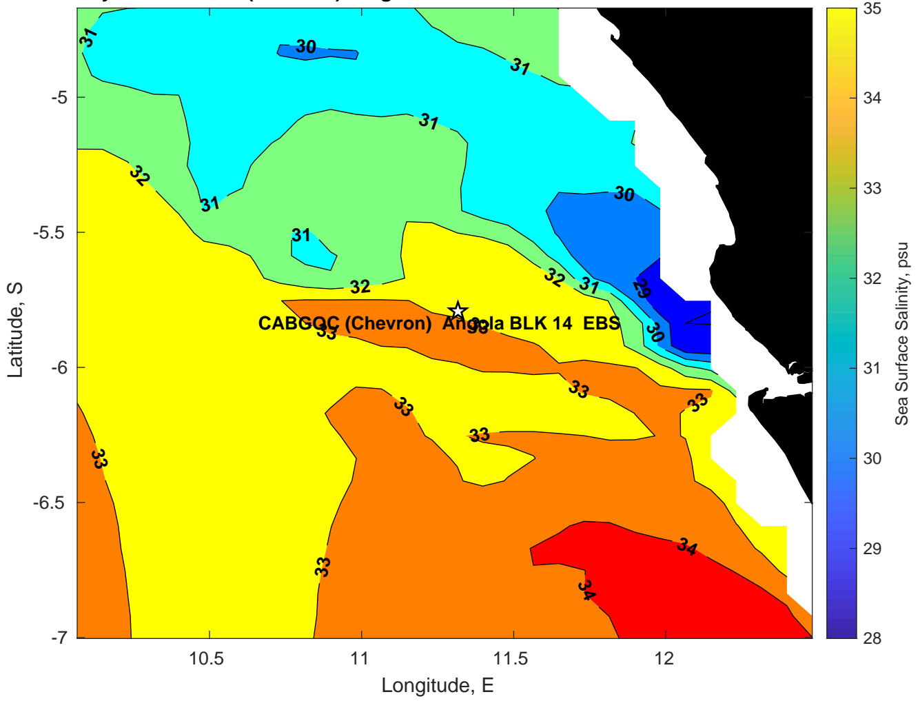
Surface Salinity for CABGOC (Chevron) Angola BLK 14 EBS at 27-Feb-2025 00:00:00
