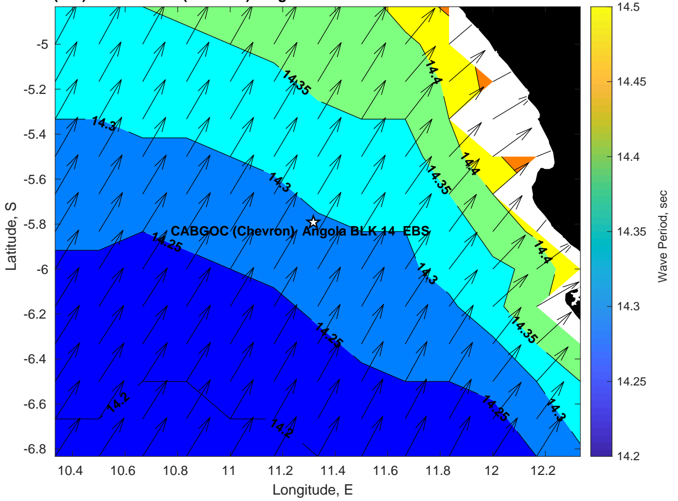
Wave Period (sec) for CABGOC (Chevron) Angola BLK 14 EBS at 28-Feb-2025 09:00:00
