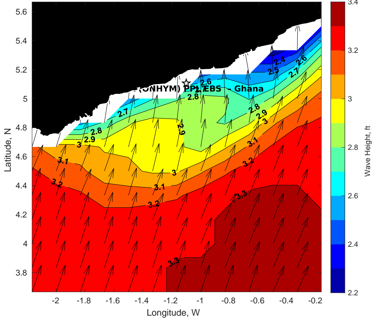
Wave Height (ft) for CSA (ONHYM) PPL EBS - Ghana at 28-Feb-2025 09:00:00
