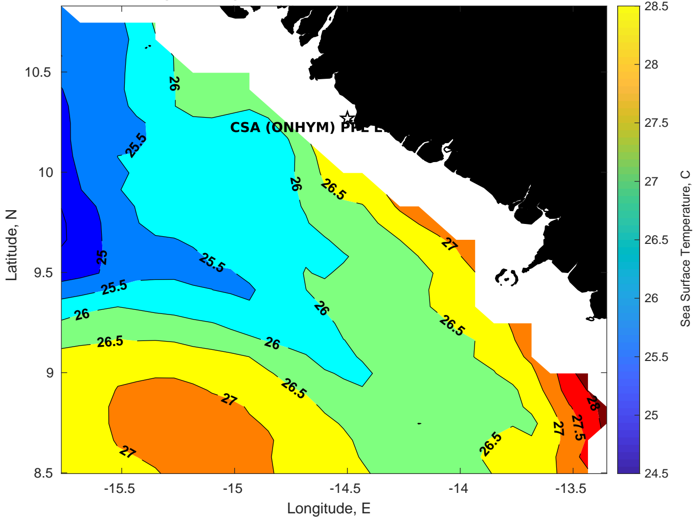
SST for CSA (ONHYM) PPL EBS - Guinea at 27-Feb-2025 00:00:00
