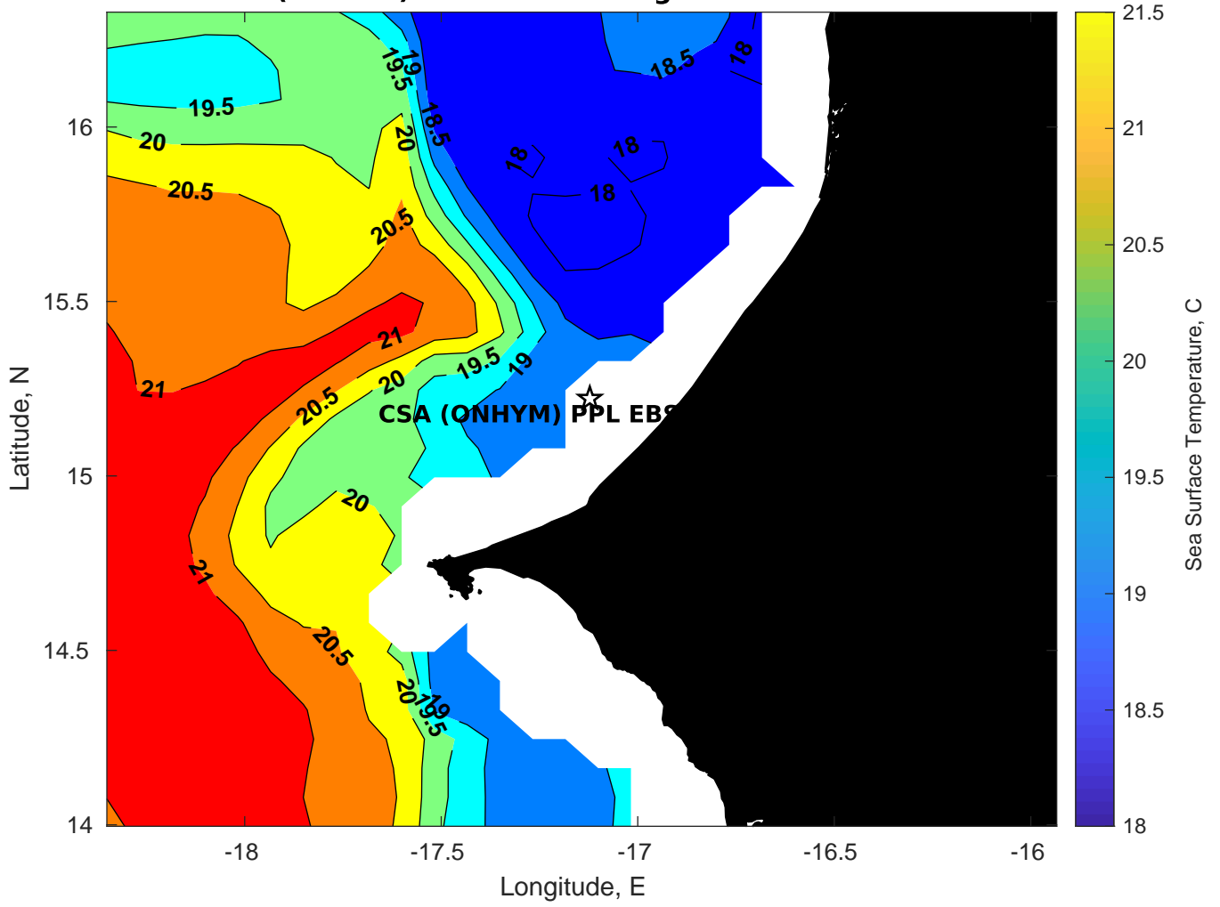
SST for CSA (ONHYM) PPL EBS - Senegal at 27-Feb-2025 00:00:00
