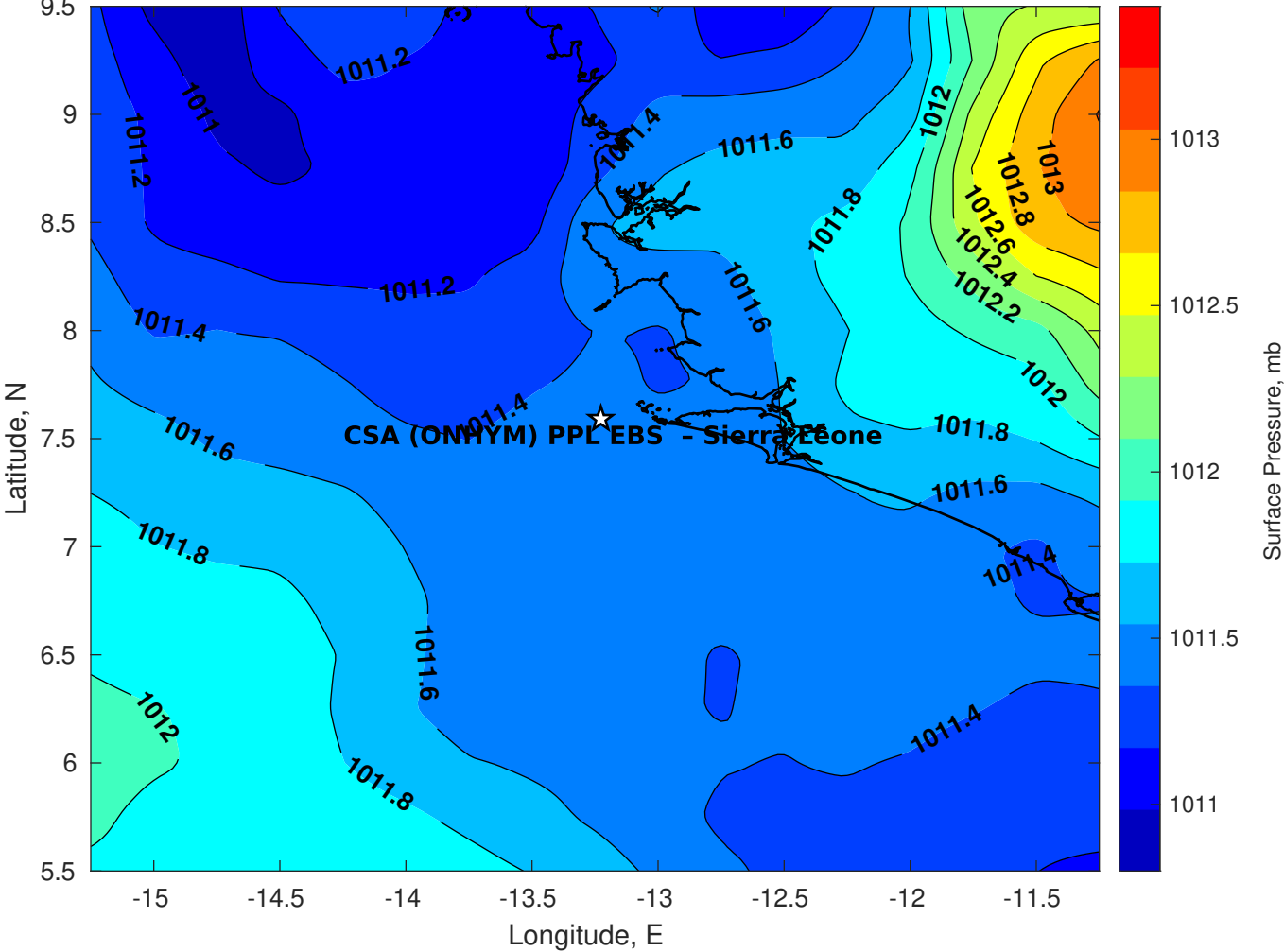
Surface Pressure (mb) for CSA (ONHYM) PPL EBS - Sierra Leone at 28-Feb-2025 00:00:00
