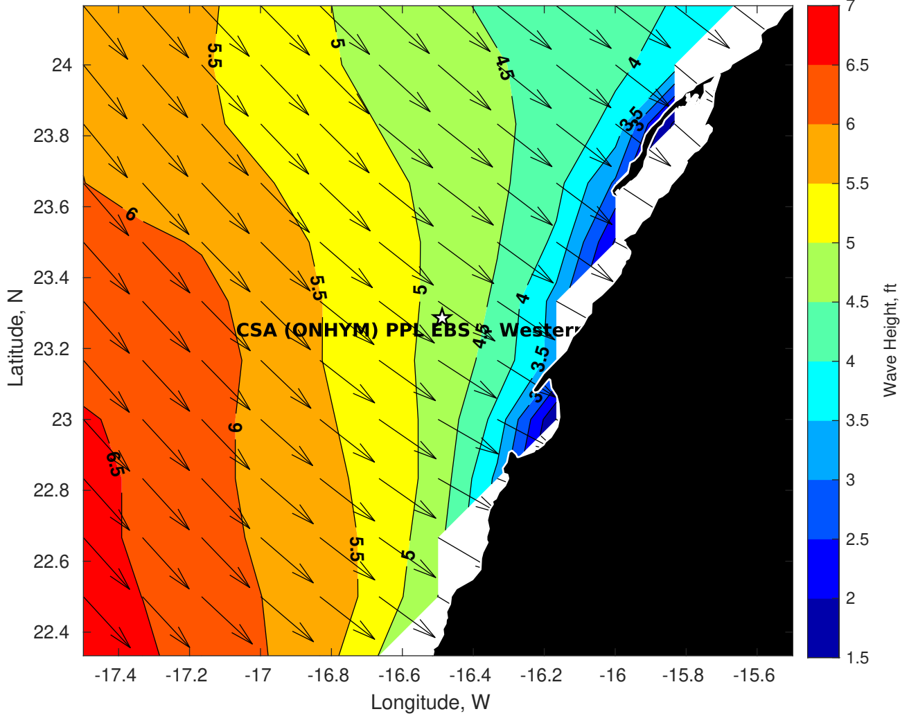
Wave Height (ft) for CSA (ONHYM) PPL EBS - Western Sahara at 28-Feb-2025 09:00:00
