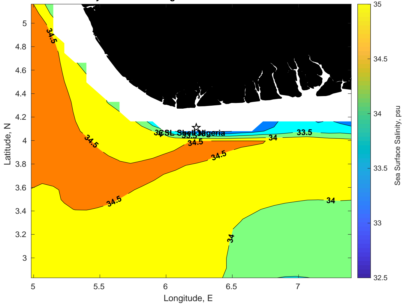
Surface Salinity for CSL Shell Nigeria at 27-Feb-2025 00:00:00
