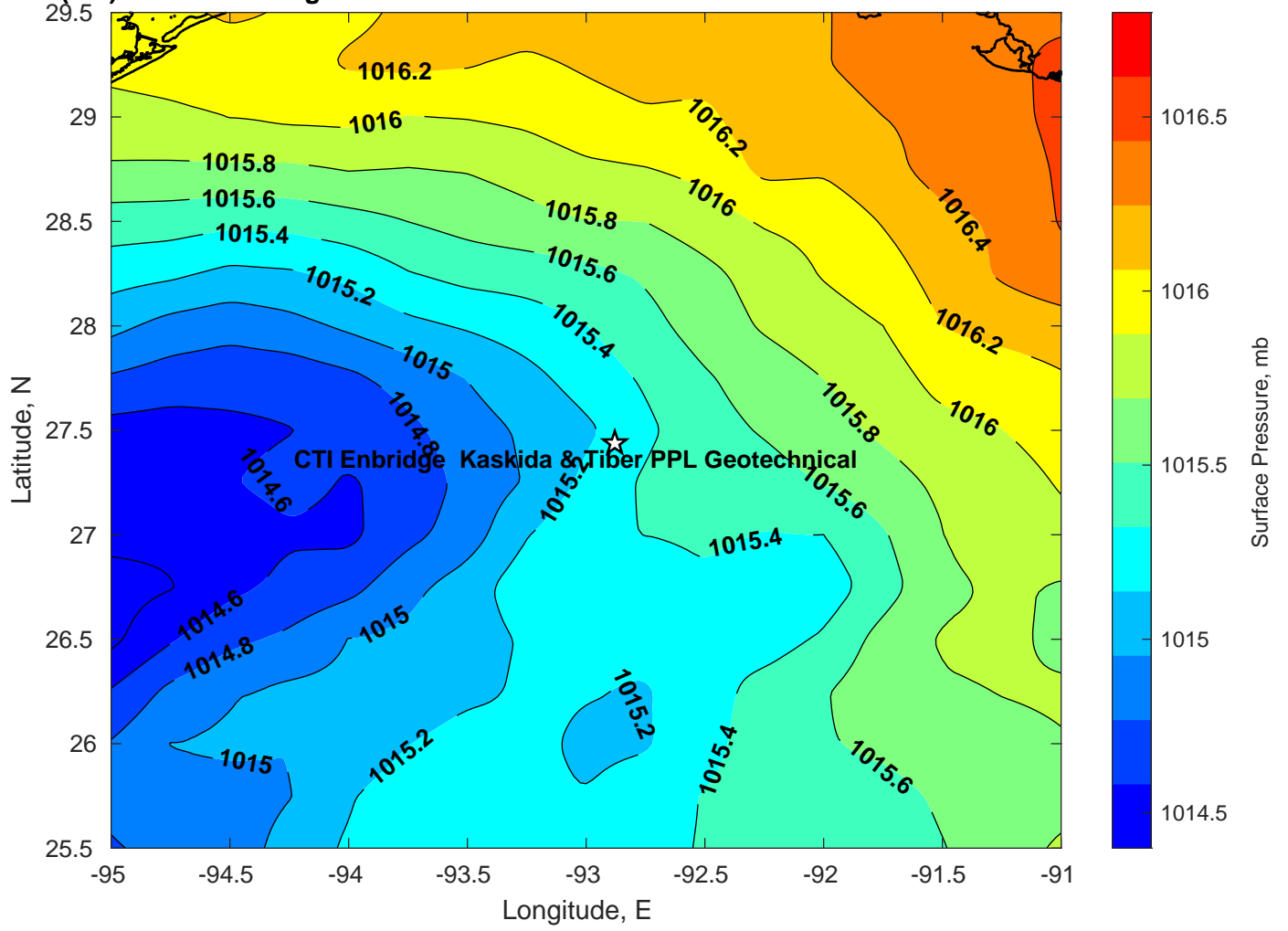
Surface Pressure (mb) for CTI Enbridge Kaskida & Tiber PPL Geotechnical at 01-Mar-2025 00:00:00
