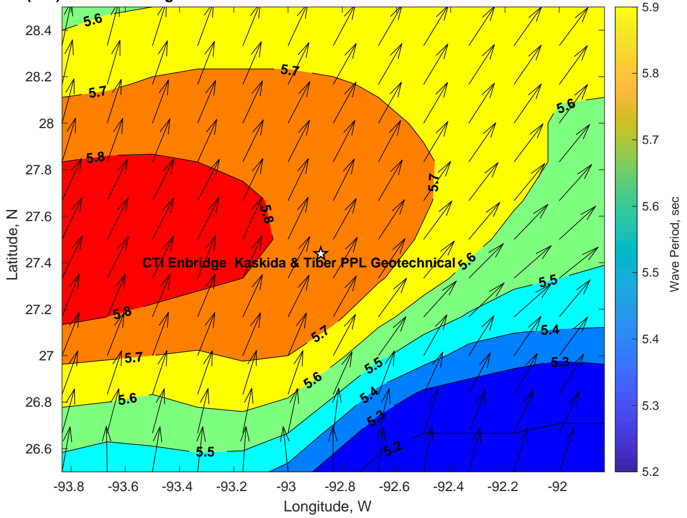
Wave Period (sec) for CTI Enbridge Kaskida & Tiber PPL Geotechnical at 28-Feb-2025 09:00:00
