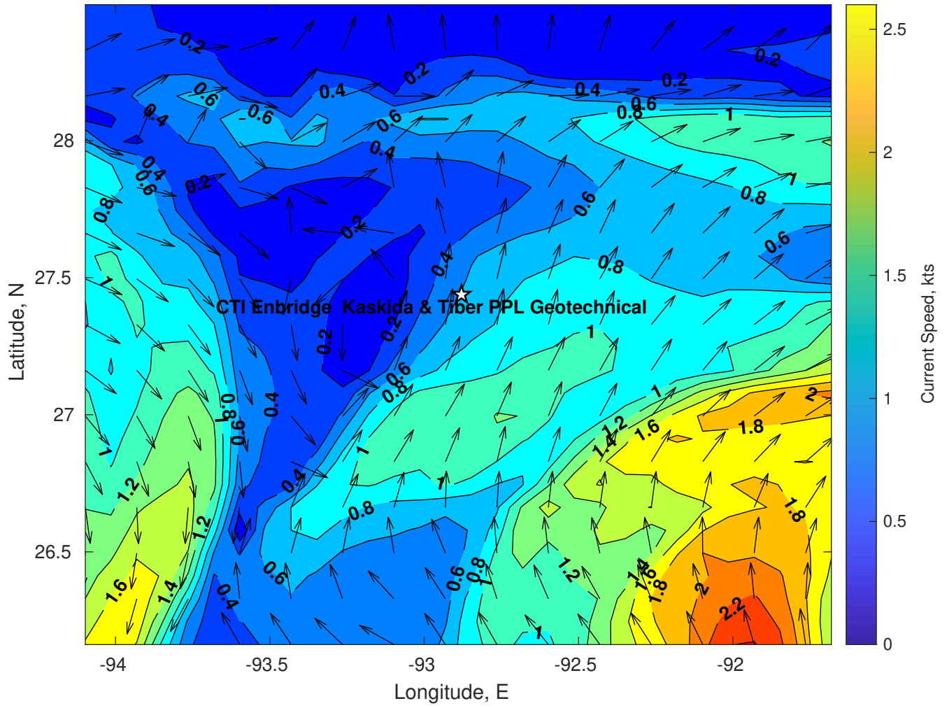
Surface Currents for CTI Enbridge Kaskida & Tiber PPL Geotechnical at 27-Feb-2025 00:00:00
