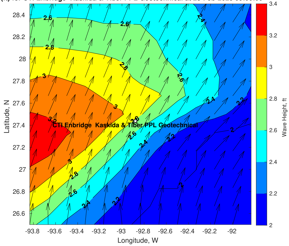
Wave Height (ft) for CTI Enbridge Kaskida & Tiber PPL Geotechnical at 28-Feb-2025 09:00:00
