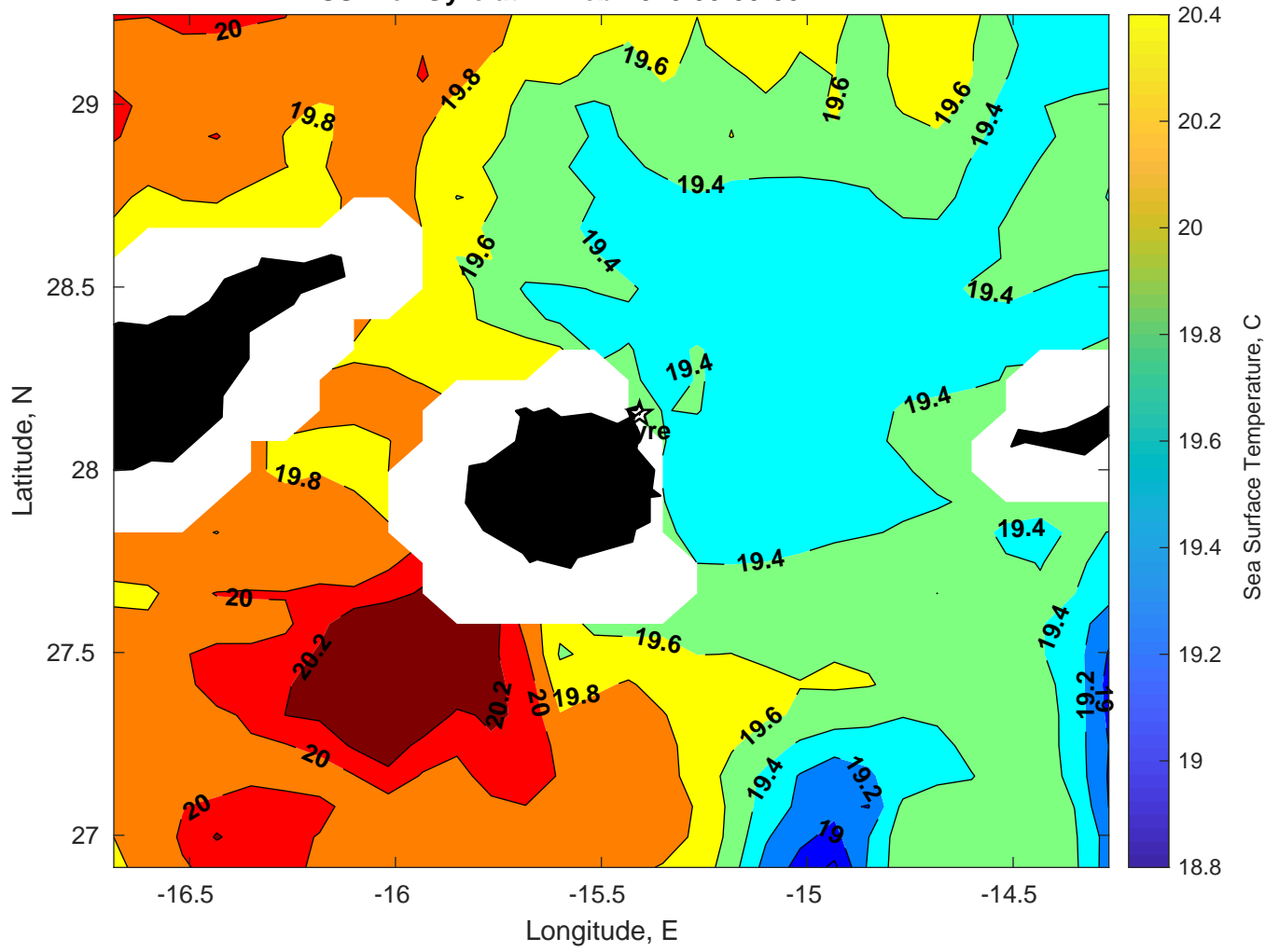
SST for Gyre at 27-Feb-2025 00:00:00
