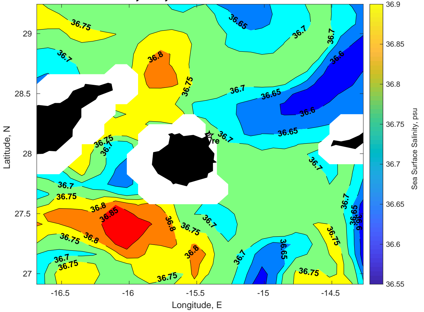
Surface Salinity for Gyre at 27-Feb-2025 00:00:00
