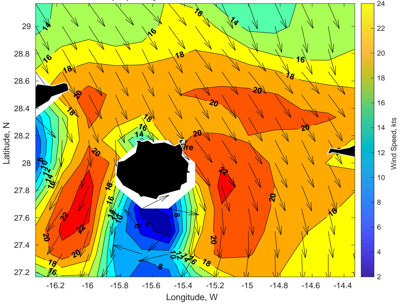
Winds (kts) for Gyre at 28-Feb-2025 09:00:00
