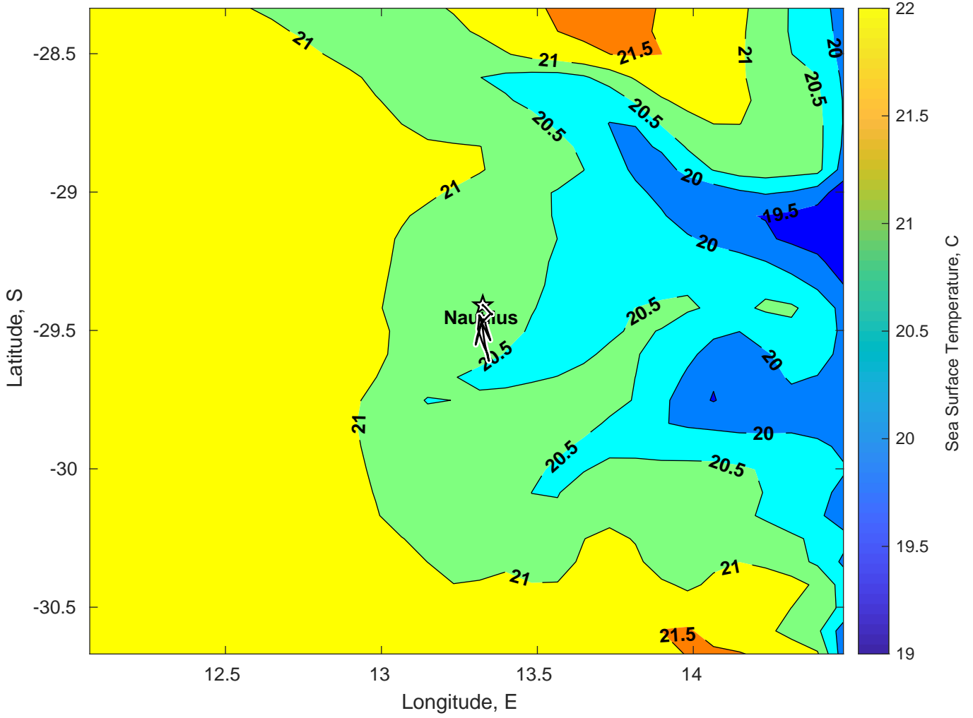
SST for Nautilus at 27-Feb-2025 00:00:00
