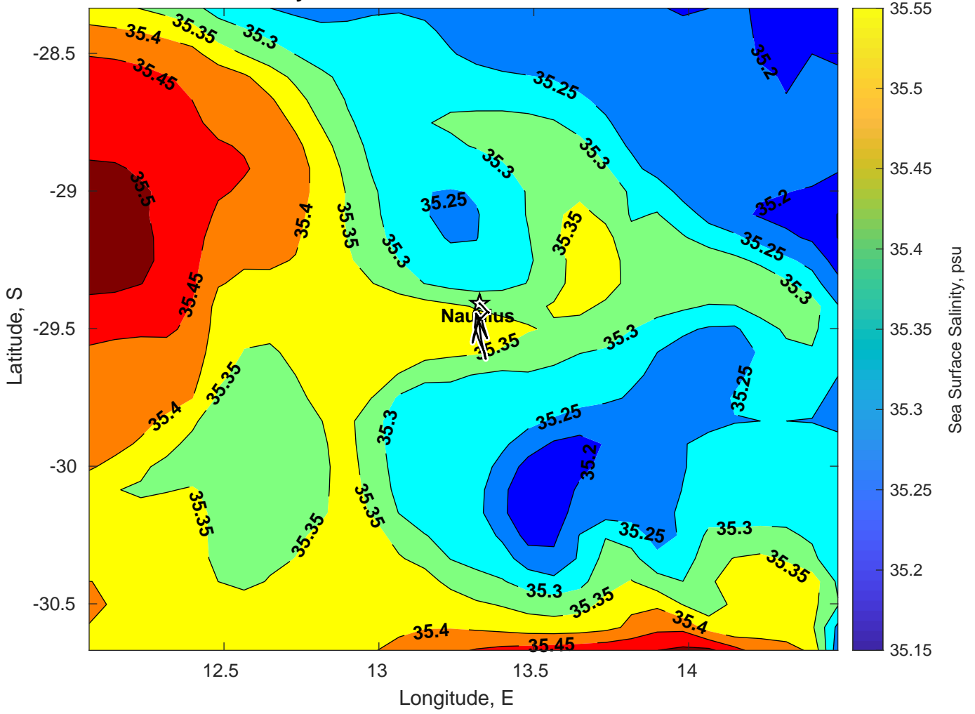
Surface Salinity for Nautilus at 27-Feb-2025 00:00:00
