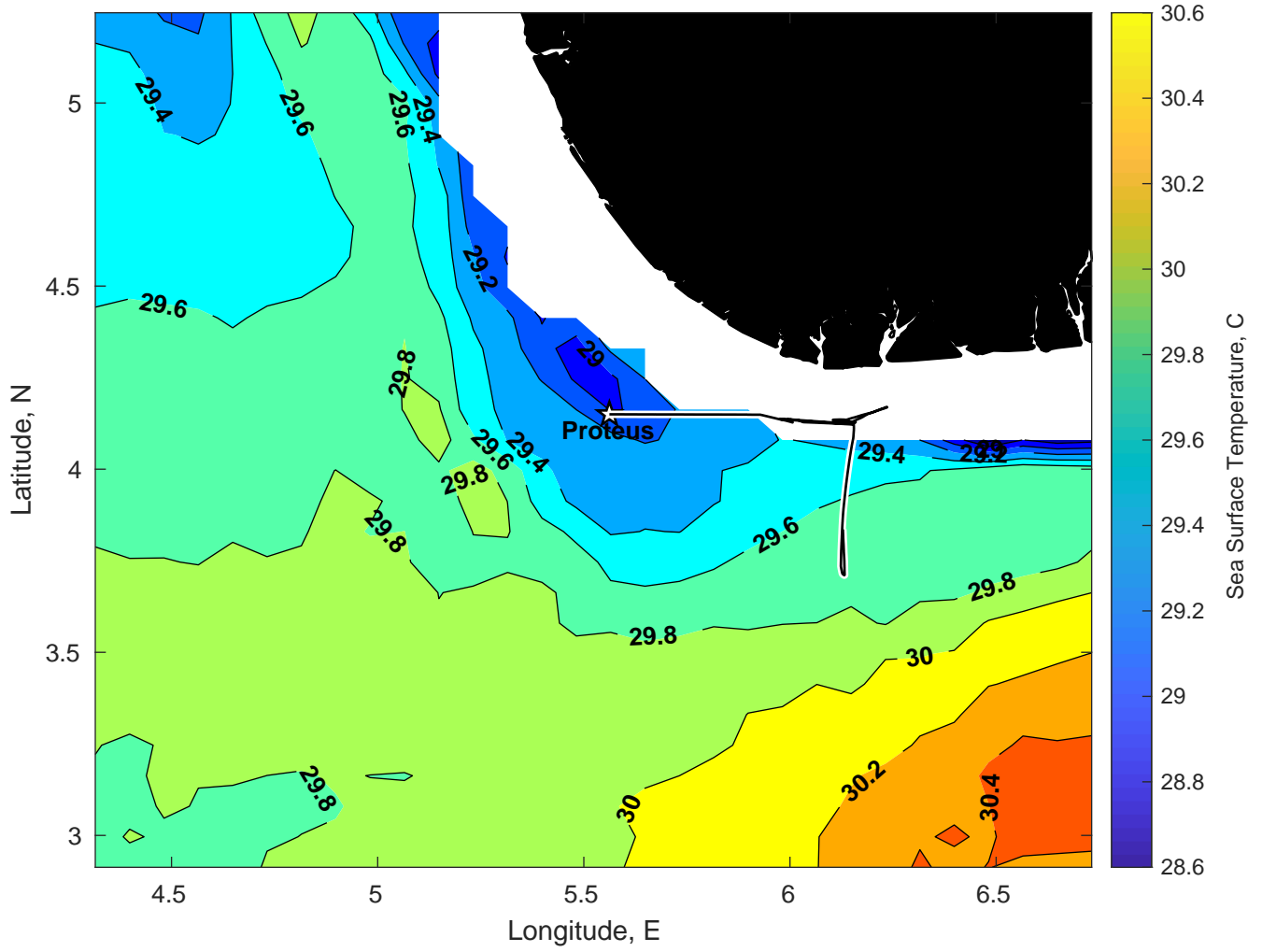
SST for Proteus at 27-Feb-2025 00:00:00
