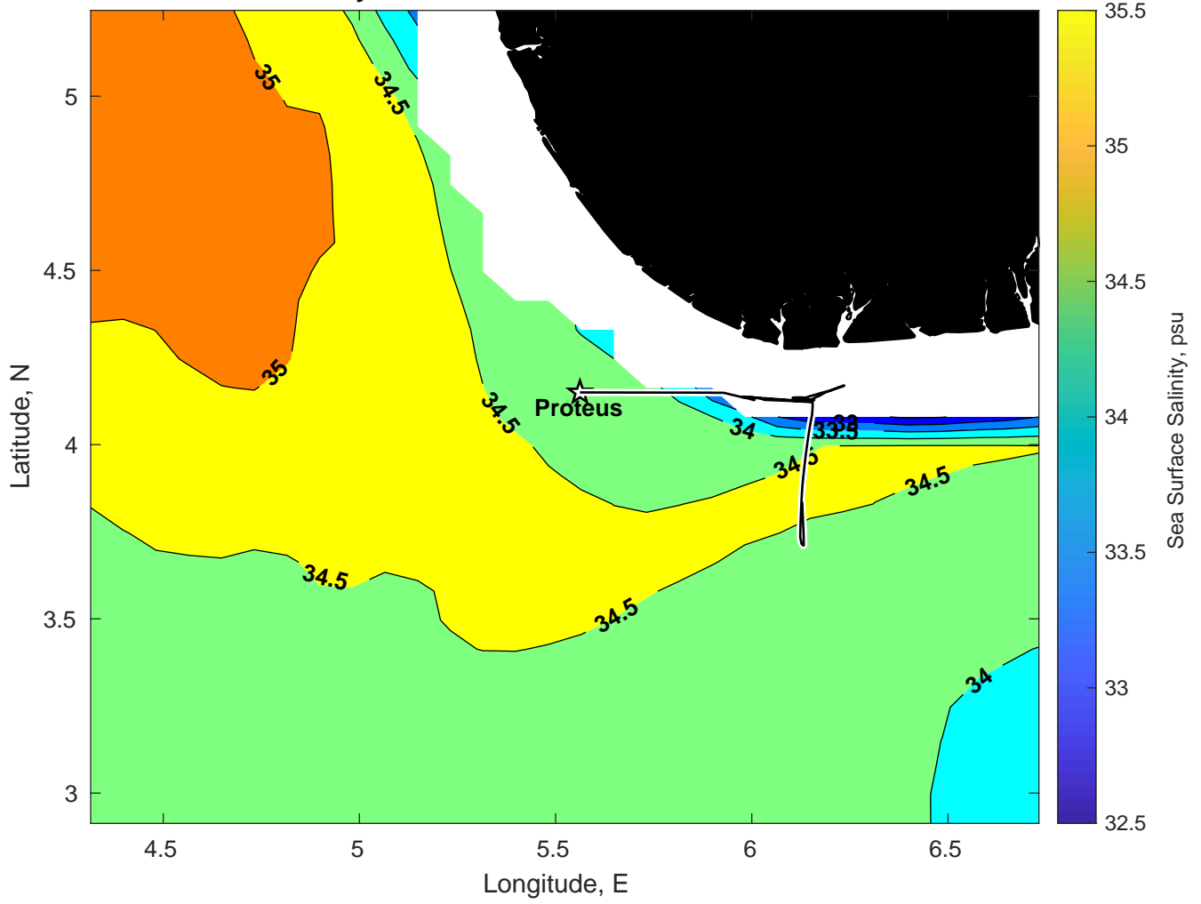
Surface Salinity for Proteus at 27-Feb-2025 00:00:00
