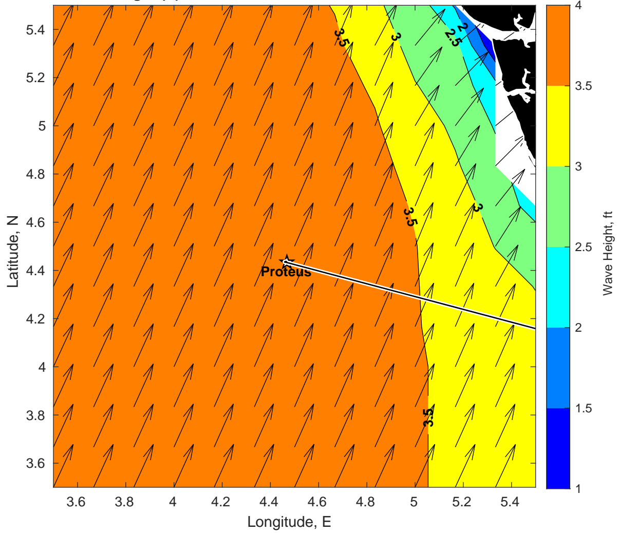
Wave Height (ft) for Proteus at 28-Feb-2025 09:00:00
