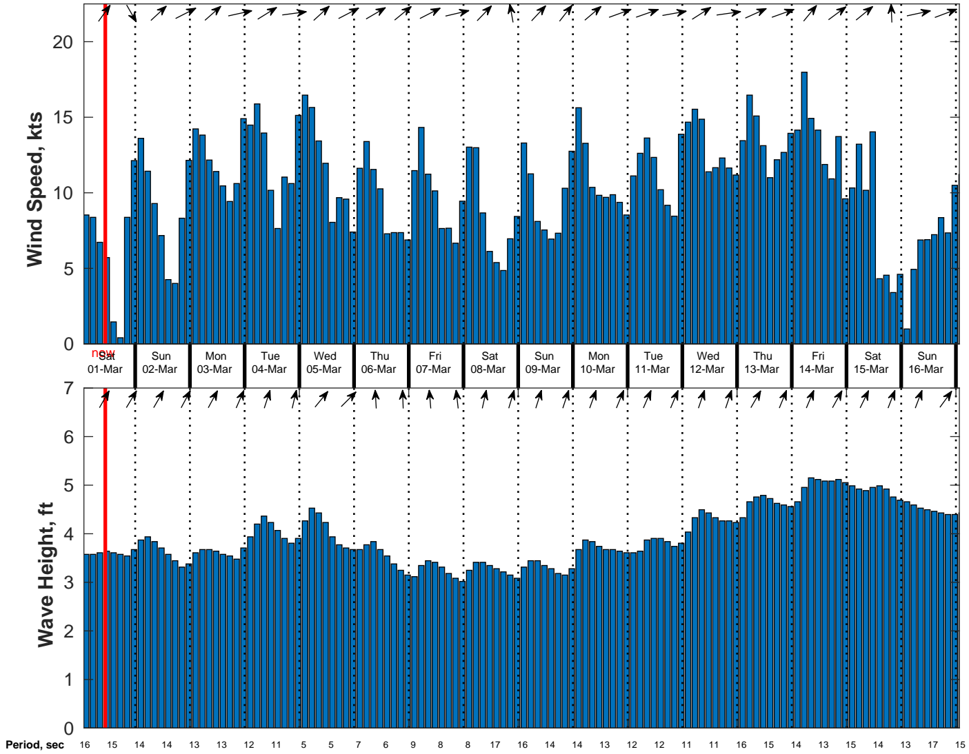
Wind & Wave Forecast for Proteus from 28-Feb-2025 01:00:00 to 16-Mar-2025 01:00:00
