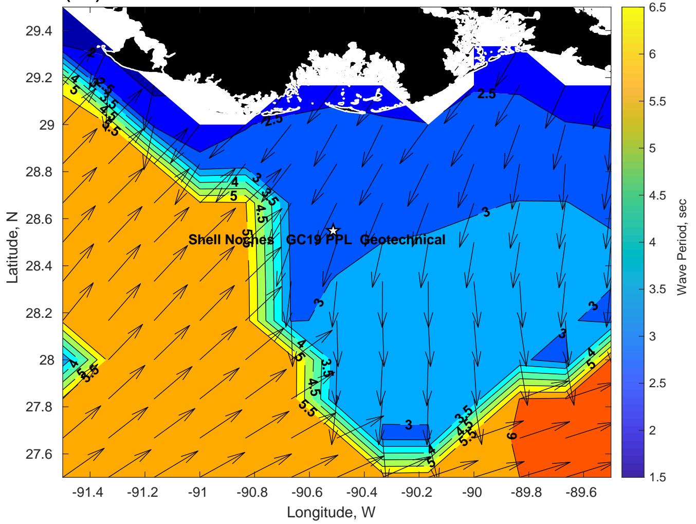
Wave Period (sec) for Shell Noches GC19 PPL Geotechnical at 28-Feb-2025 09:00:00
