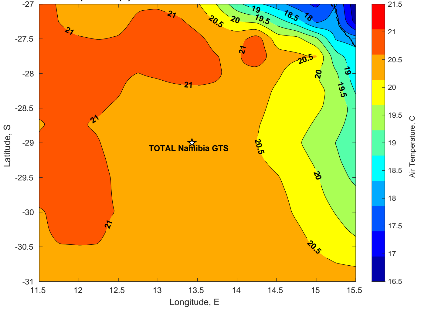
Air Temperature (C) for TOTAL Namibia GTS at 28-Feb-2025
