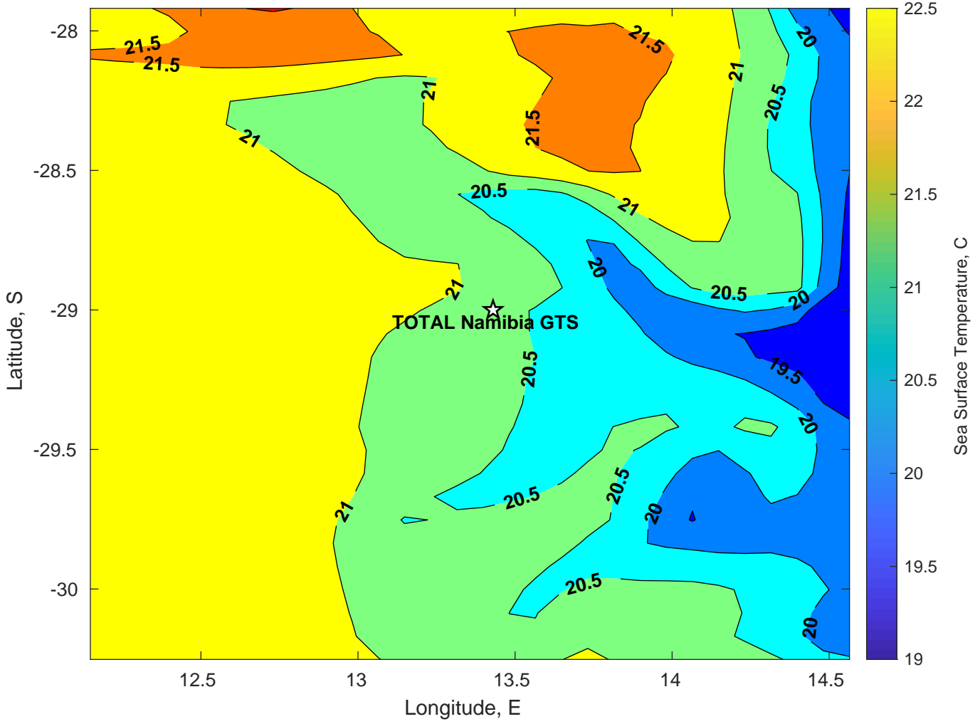
SST for TOTAL Namibia GTS at 27-Feb-2025 00:00:00
