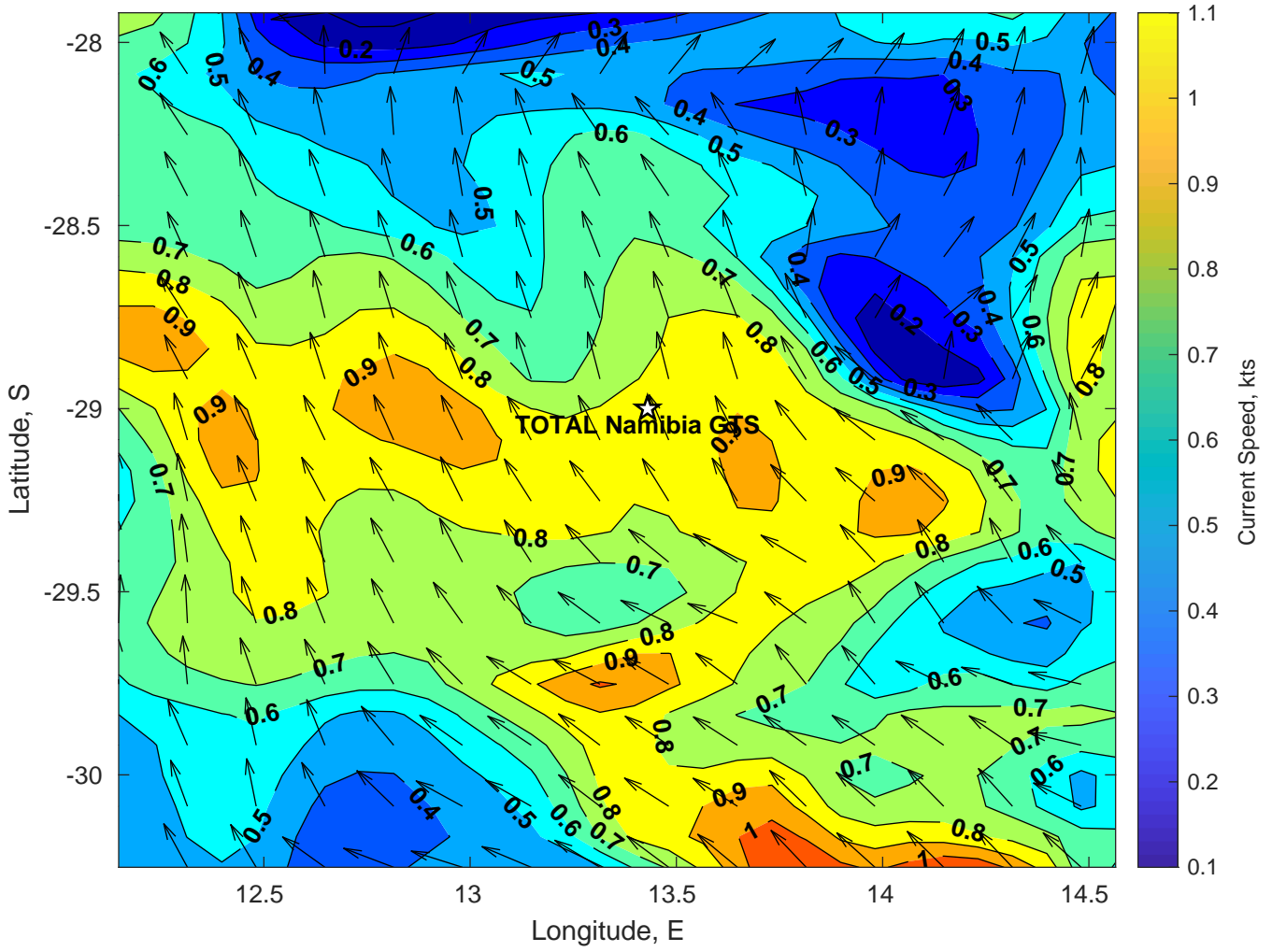
Surface Currents for TOTAL Namibia GTS at 27-Feb-2025 00:00:00
