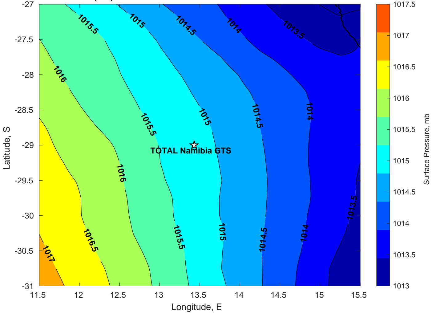
Surface Pressure (mb) for TOTAL Namibia GTS at 28-Feb-2025 00:00:00
