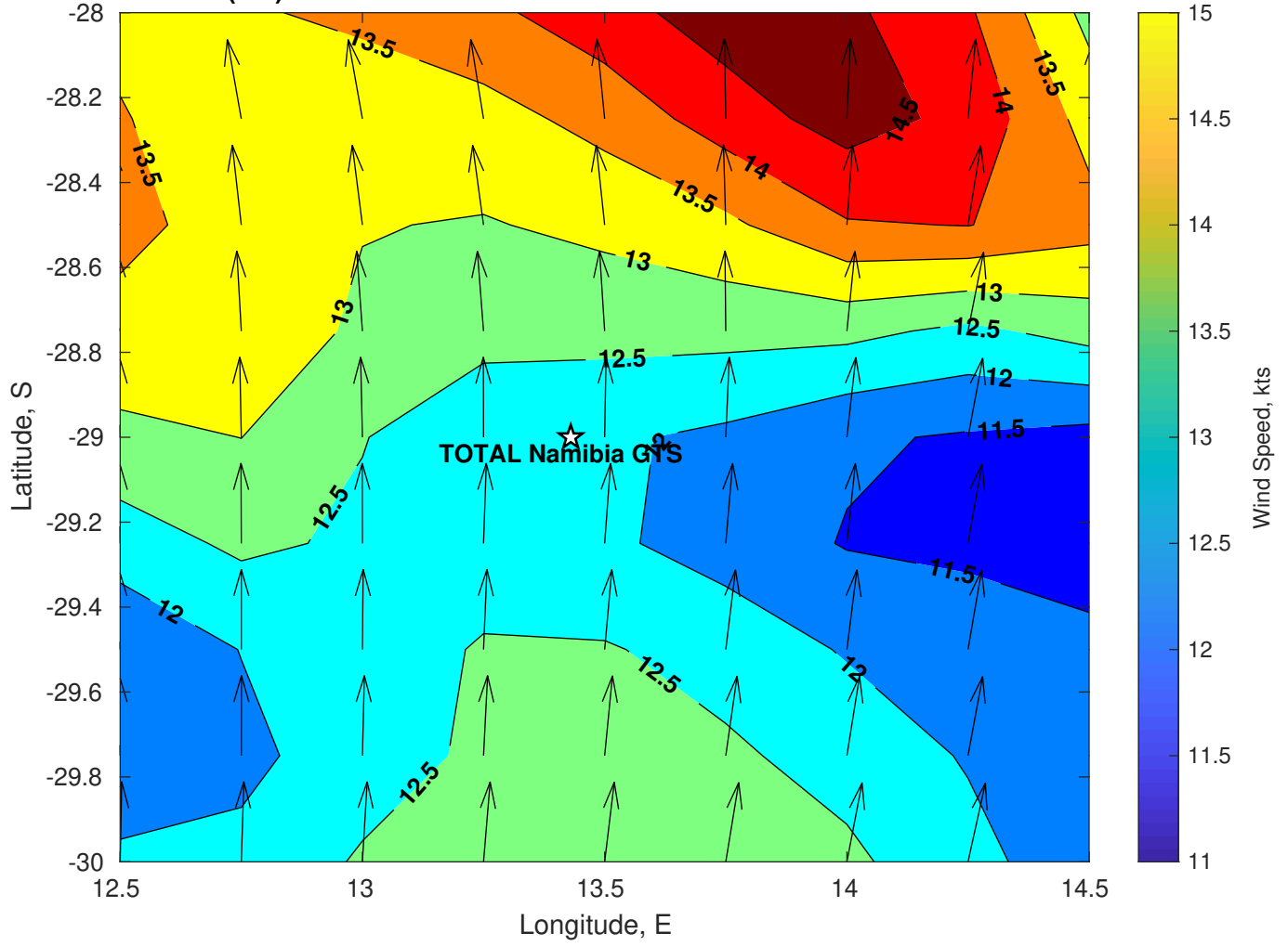
Winds (kts) for TOTAL Namibia GTS at 28-Feb-2025 09:00:00
