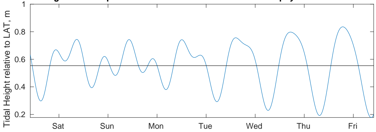
Tidal Currents and Heights for Tampnet P2378 South Texas Cable Route Geophysical at 20250228
