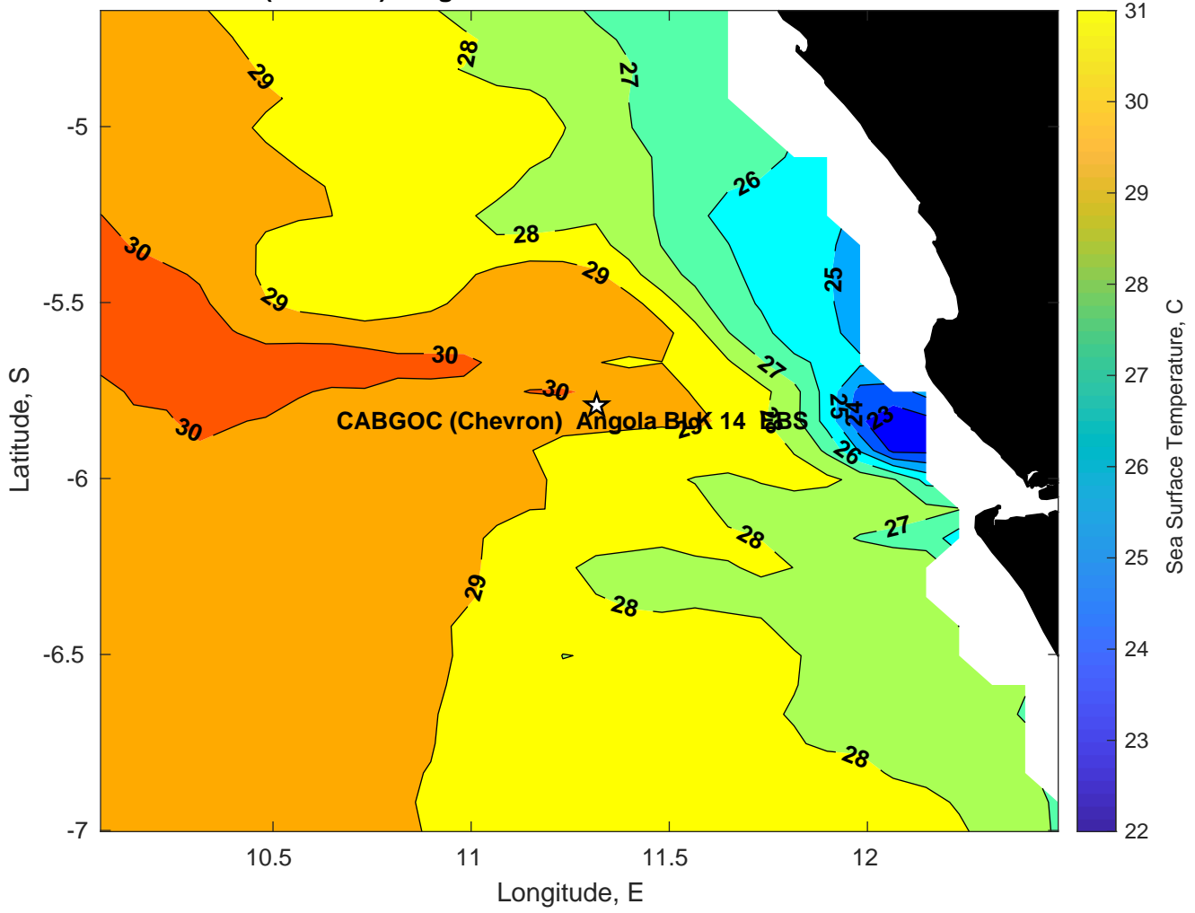
SST for CABGOC (Chevron) Angola BLK 14 EBS at 28-Feb-2025 00:00:00
