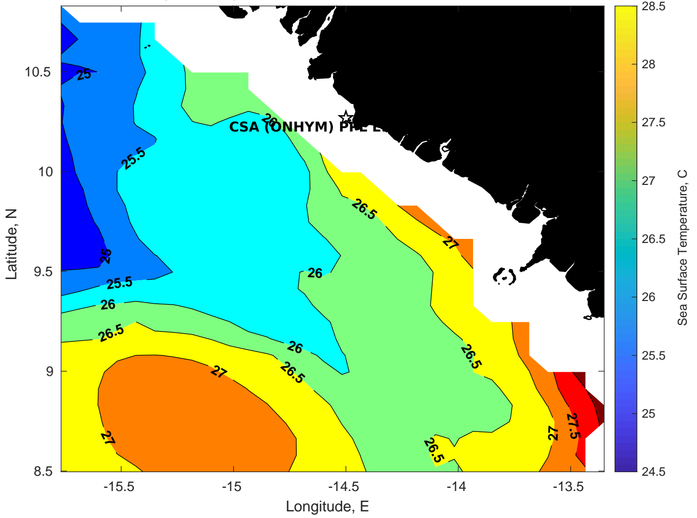
SST for CSA (ONHYM) PPL EBS - Guinea at 28-Feb-2025 00:00:00
